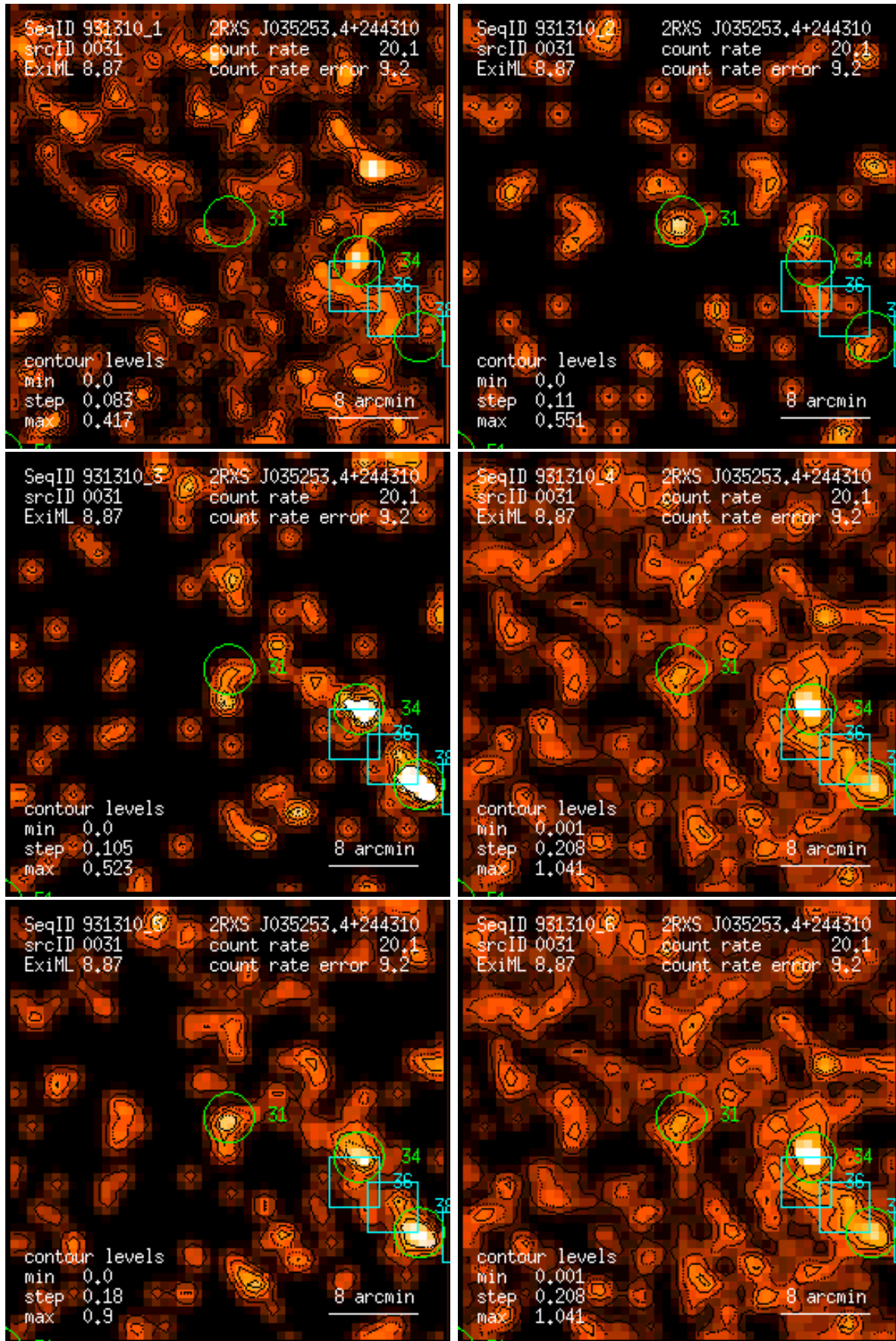
Figure 31: RASS 931310: detection 0031: band rate images, Gaussian filter: (1) PSPC channels 11 – 41, (2) 52 – 90, (3) 91 – 201, (4) 11 – 235, (5) 52 – 201, (6) 11 – 201. Broad band rates in counts/ks. Band rate contour levels in counts/ks/arcmin 2 .
