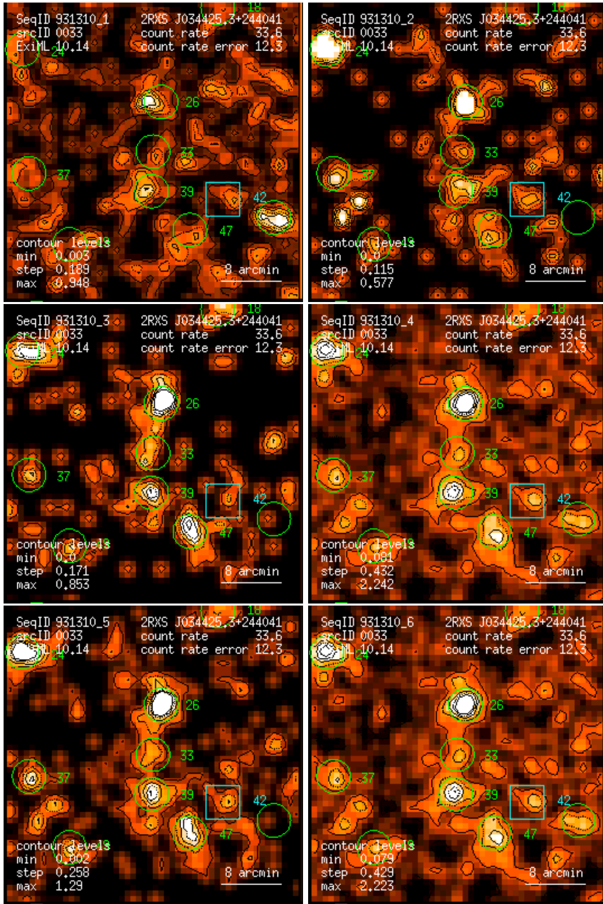
Figure 33: RASS 931310: detection 0033: band rate images, Gaussian filter: (1) PSPC channels 11 – 41, (2) 52 – 90, (3) 91 – 201, (4) 11 – 235, (5) 52 – 201, (6) 11 – 201. Broad band rates in counts/ks. Band rate contour levels in counts/ks/arcmin 2 .
