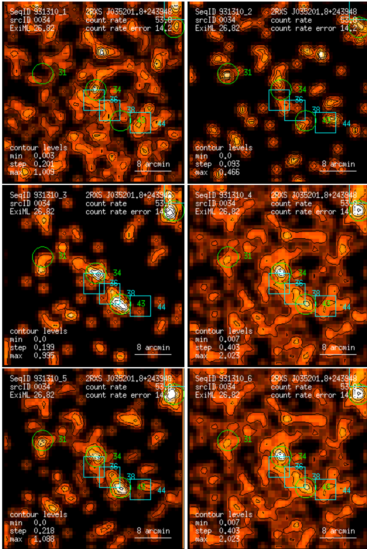
Figure 34: RASS 931310: detection 0034: band rate images, Gaussian filter: (1) PSPC channels 11 – 41, (2) 52 – 90, (3) 91 – 201, (4) 11 – 235, (5) 52 – 201, (6) 11 – 201. Broad band rates in counts/ks. Band rate contour levels in counts/ks/arcmin 2 .
