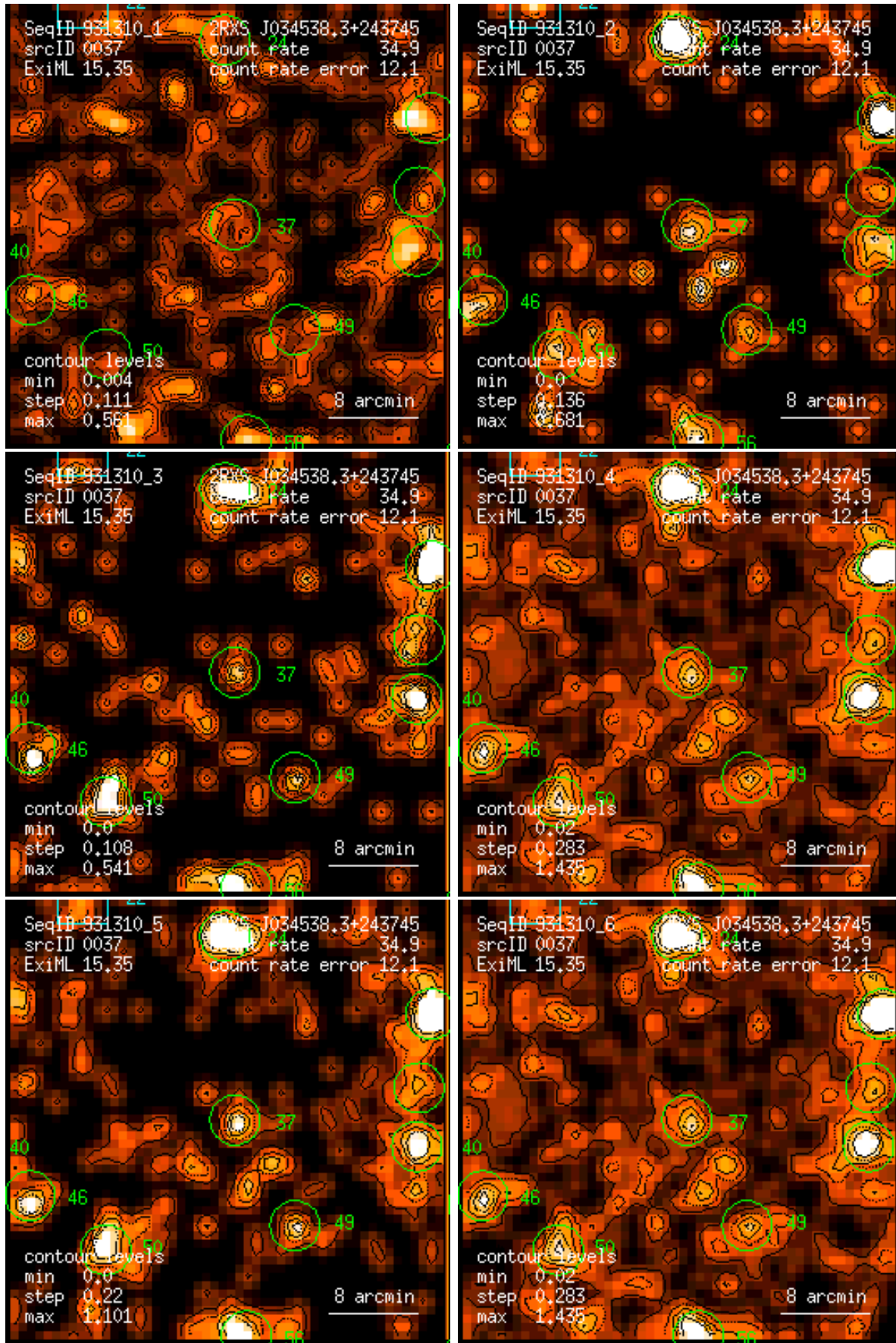
Figure 37: RASS 931310: detection 0037: band rate images, Gaussian filter: (1) PSPC channels 11 – 41, (2) 52 – 90, (3) 91 – 201, (4) 11 – 235, (5) 52 – 201, (6) 11 – 201. Broad band rates in counts/ks. Band rate contour levels in counts/ks/arcmin 2 .
