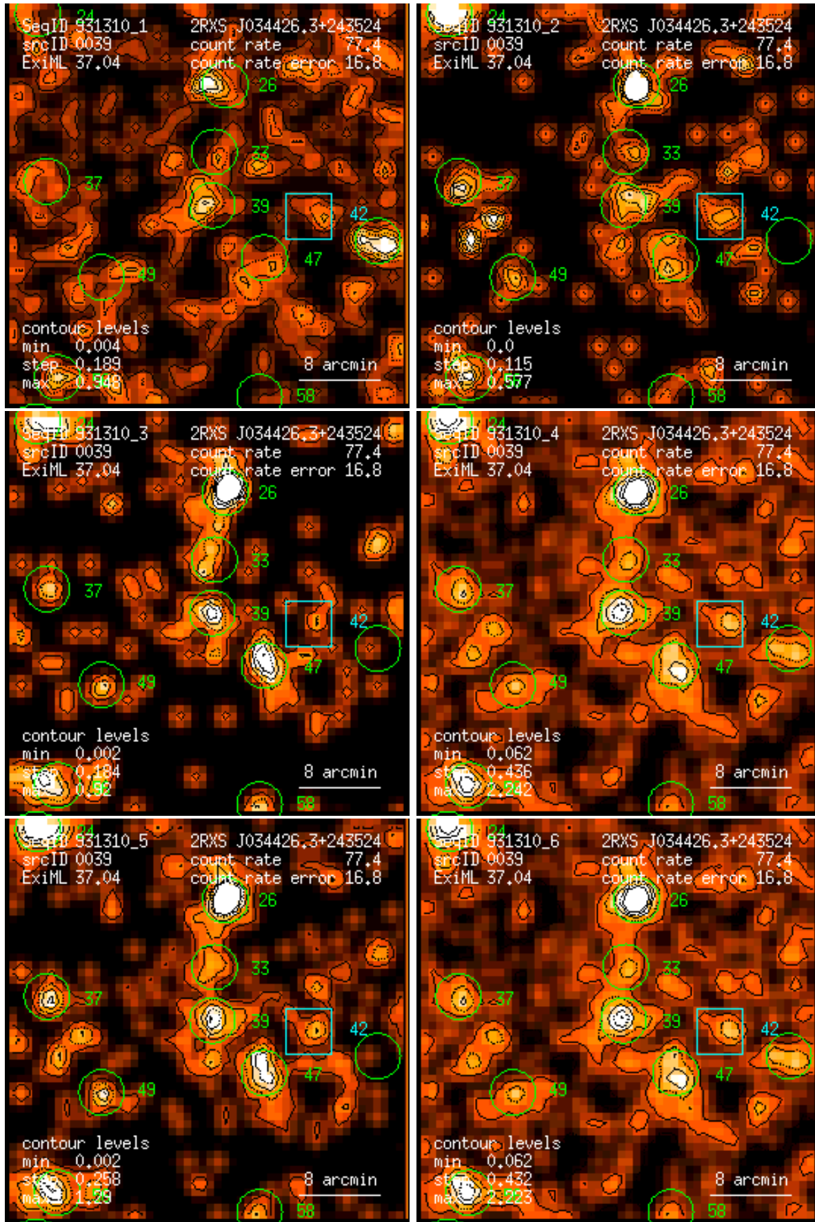
Figure 39: RASS 931310: detection 0039: band rate images, Gaussian filter: (1) PSPC channels 11 – 41, (2) 52 – 90, (3) 91 – 201, (4) 11 – 235, (5) 52 – 201, (6) 11 – 201. Broad band rates in counts/ks. Band rate contour levels in counts/ks/arcmin 2 .
