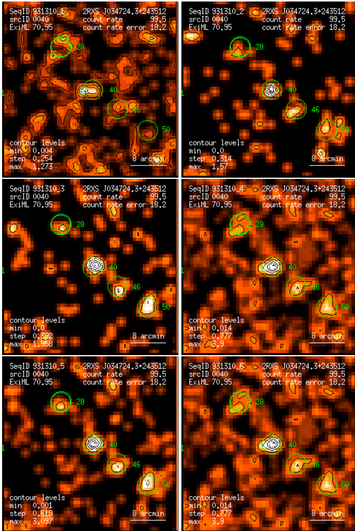
Figure 40: RASS 931310: detection 0040: band rate images, Gaussian filter: (1) PSPC channels 11 – 41, (2) 52 – 90, (3) 91 – 201, (4) 11 – 235, (5) 52 – 201, (6) 11 – 201. Broad band rates in counts/ks. Band rate contour levels in counts/ks/arcmin 2 .
