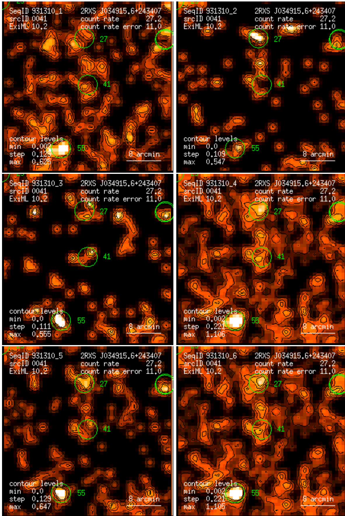
Figure 41: RASS 931310: detection 0041: band rate images, Gaussian filter: (1) PSPC channels 11 – 41, (2) 52 – 90, (3) 91 – 201, (4) 11 – 235, (5) 52 – 201, (6) 11 – 201. Broad band rates in counts/ks. Band rate contour levels in counts/ks/arcmin 2 .
