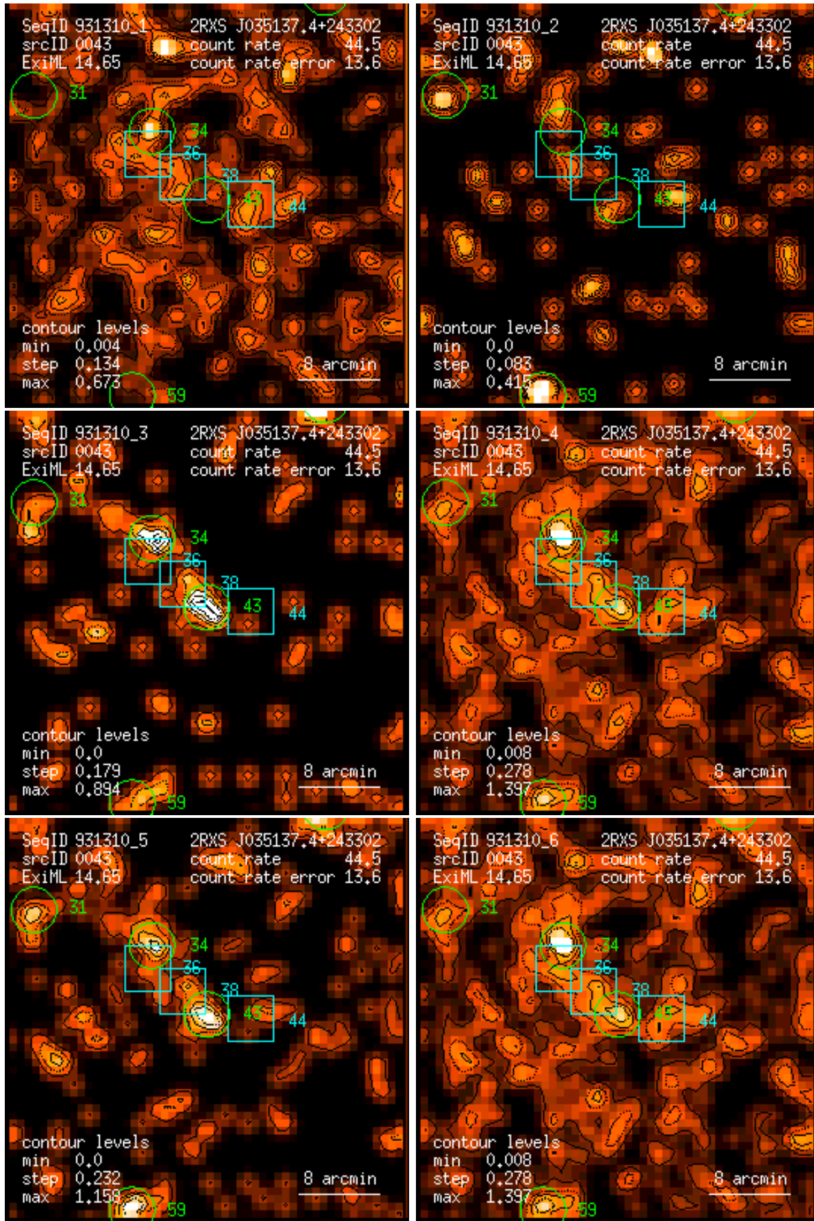
Figure 43: RASS 931310: detection 0043: band rate images, Gaussian filter: (1) PSPC channels 11 – 41, (2) 52 – 90, (3) 91 – 201, (4) 11 – 235, (5) 52 – 201, (6) 11 – 201. Broad band rates in counts/ks. Band rate contour levels in counts/ks/arcmin 2 .
