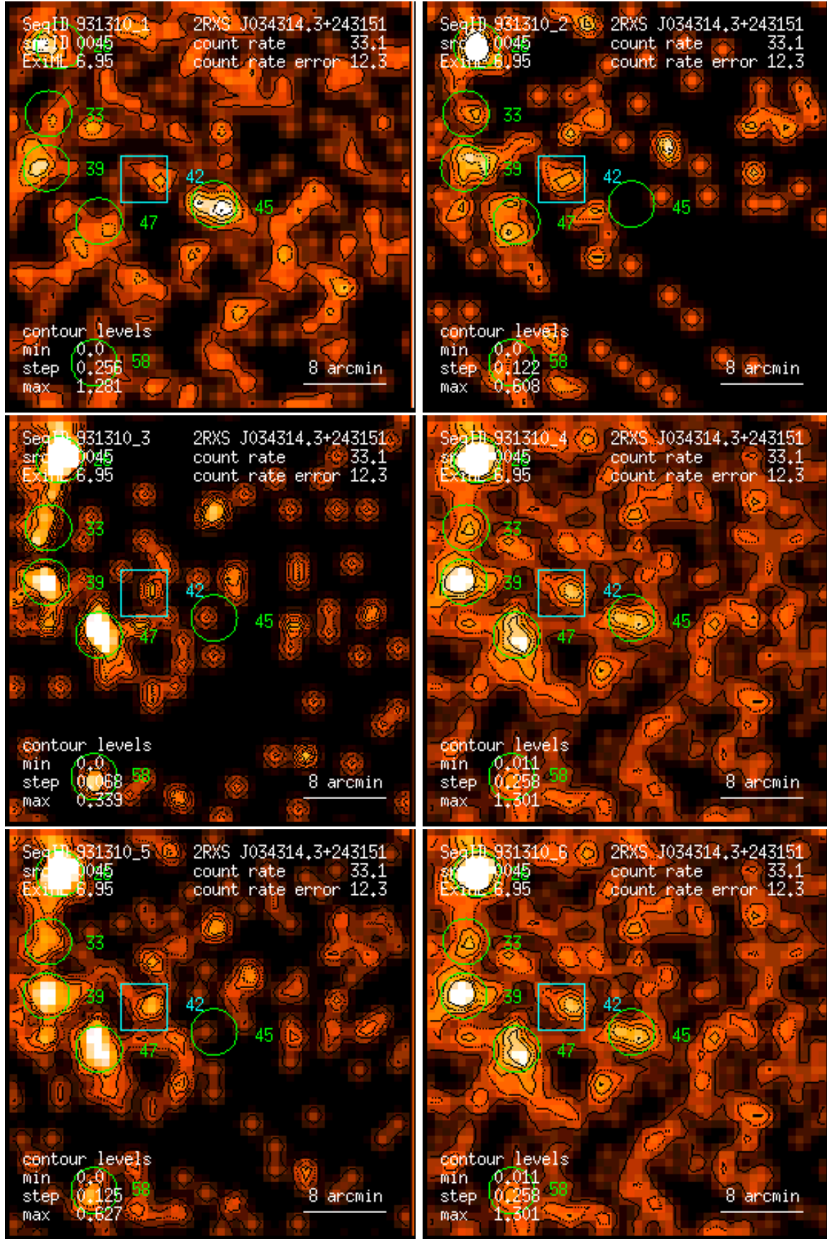
Figure 45: RASS 931310: detection 0045: band rate images, Gaussian filter: (1) PSPC channels 11 – 41, (2) 52 – 90, (3) 91 – 201, (4) 11 – 235, (5) 52 – 201, (6) 11 – 201. Broad band rates in counts/ks. Band rate contour levels in counts/ks/arcmin 2 .
