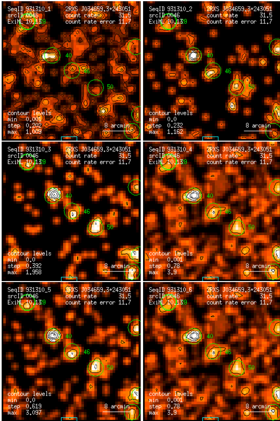
Figure 46: RASS 931310: detection 0046: band rate images, Gaussian filter: (1) PSPC channels 11 – 41, (2) 52 – 90, (3) 91 – 201, (4) 11 – 235, (5) 52 – 201, (6) 11 – 201. Broad band rates in counts/ks. Band rate contour levels in counts/ks/arcmin 2 .
