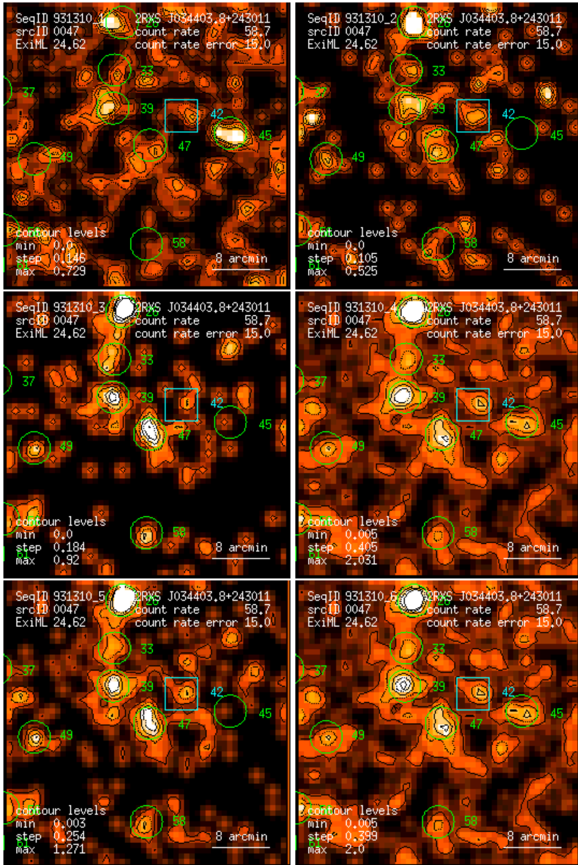
Figure 47: RASS 931310: detection 0047: band rate images, Gaussian filter: (1) PSPC channels 11 – 41, (2) 52 – 90, (3) 91 – 201, (4) 11 – 235, (5) 52 – 201, (6) 11 – 201. Broad band rates in counts/ks. Band rate contour levels in counts/ks/arcmin 2 .
