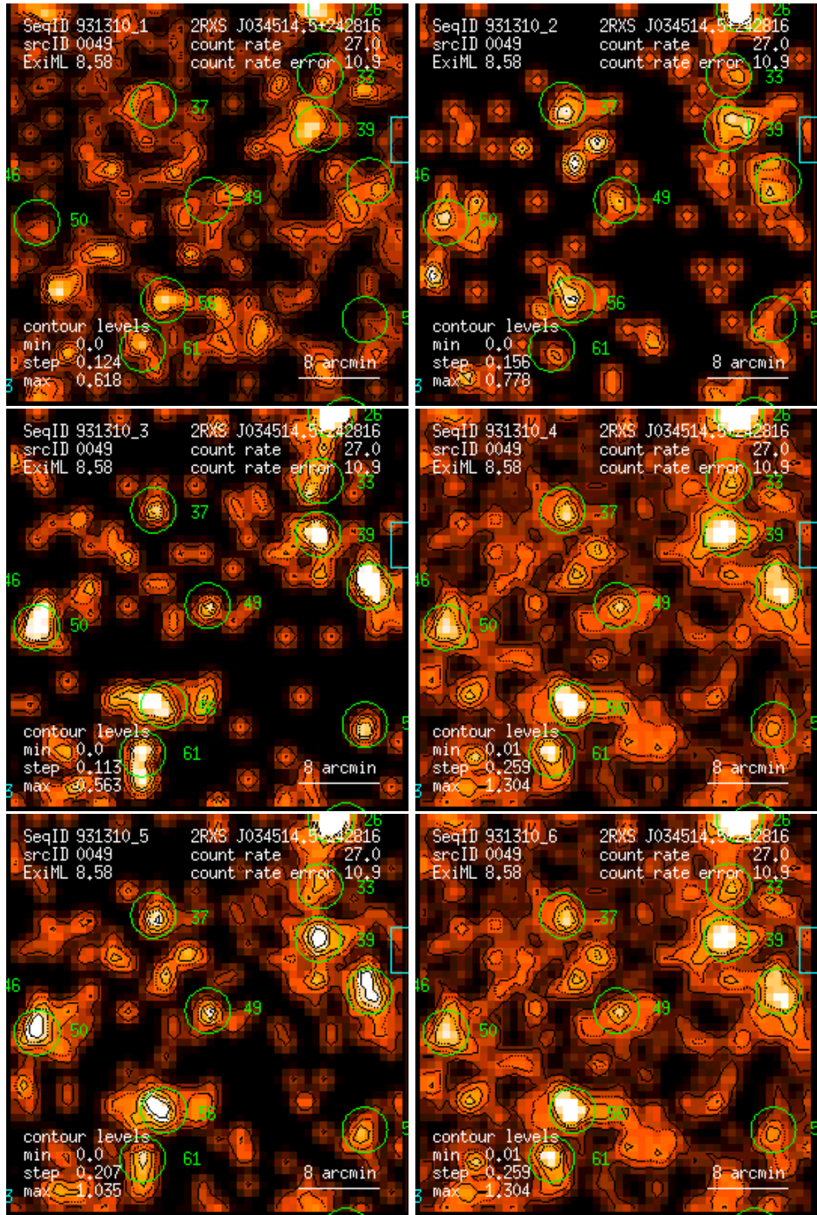
Figure 49: RASS 931310: detection 0049: band rate images, Gaussian filter: (1) PSPC channels 11 – 41, (2) 52 – 90, (3) 91 – 201, (4) 11 – 235, (5) 52 – 201, (6) 11 – 201. Broad band rates in counts/ks. Band rate contour levels in counts/ks/arcmin 2 .
