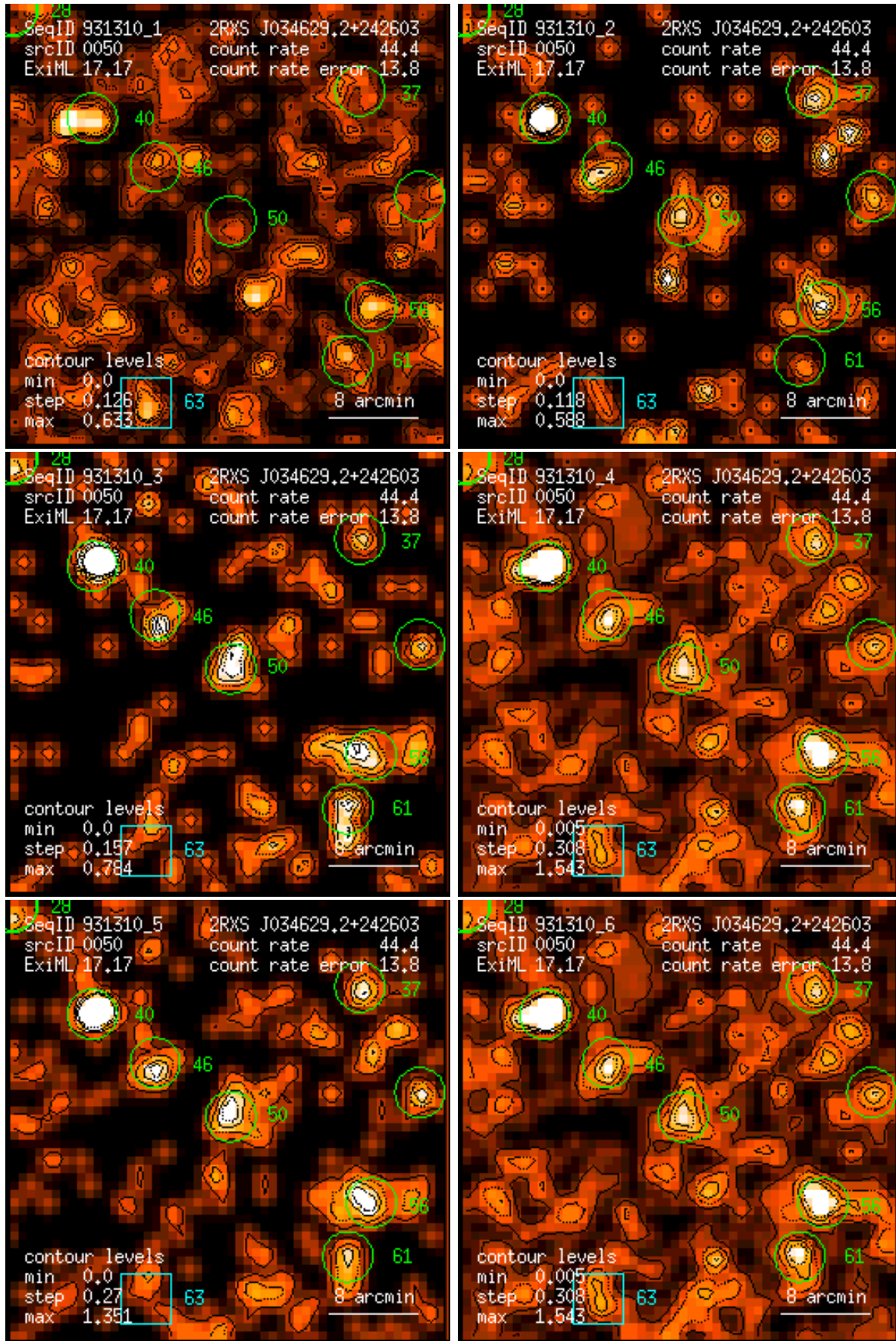
Figure 50: RASS 931310: detection 0050: band rate images, Gaussian filter: (1) PSPC channels 11 – 41, (2) 52 – 90, (3) 91 – 201, (4) 11 – 235, (5) 52 – 201, (6) 11 – 201. Broad band rates in counts/ks. Band rate contour levels in counts/ks/arcmin 2 .
