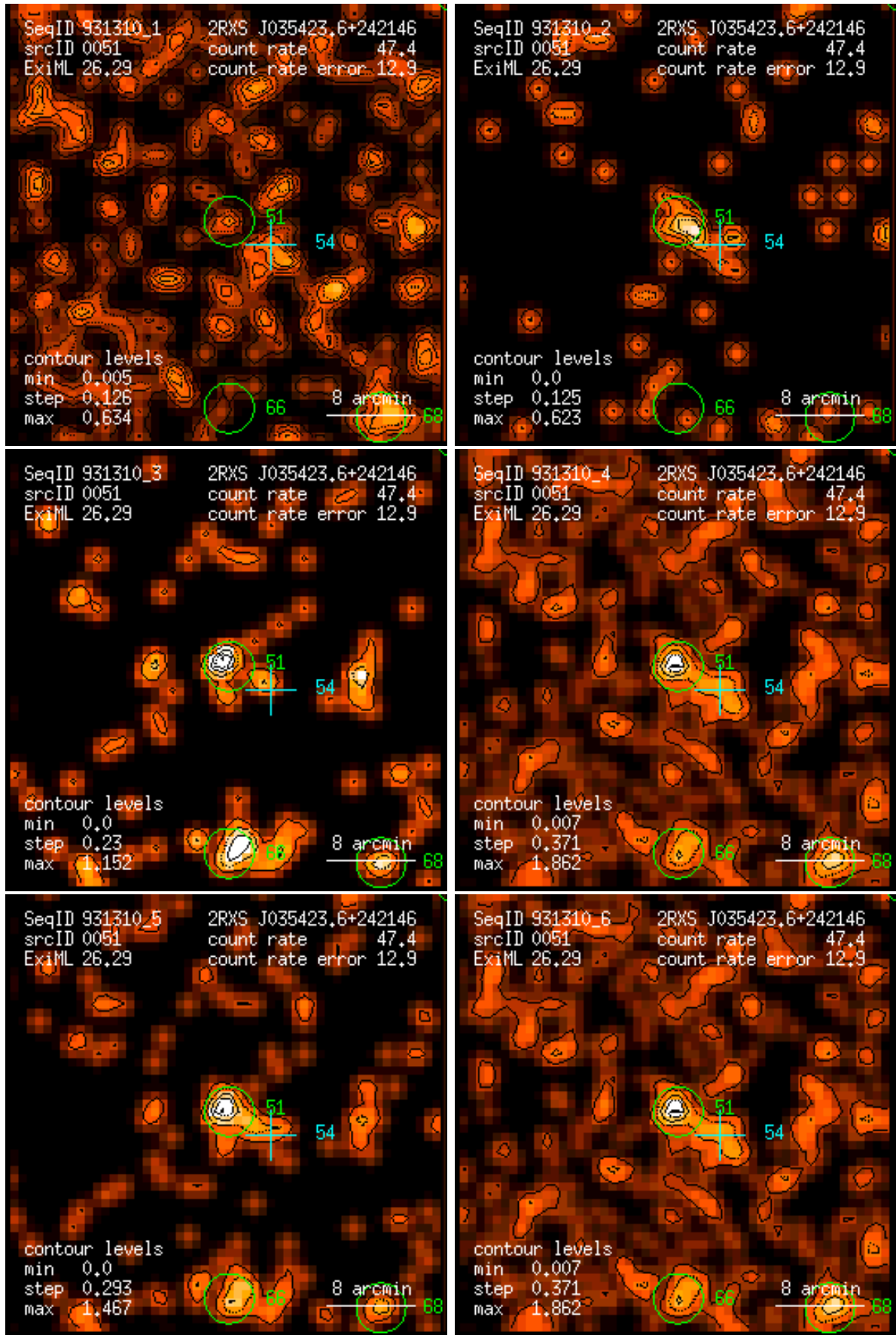
Figure 51: RASS 931310: detection 0051: band rate images, Gaussian filter: (1) PSPC channels 11 – 41, (2) 52 – 90, (3) 91 – 201, (4) 11 – 235, (5) 52 – 201, (6) 11 – 201. Broad band rates in counts/ks. Band rate contour levels in counts/ks/arcmin 2 .
