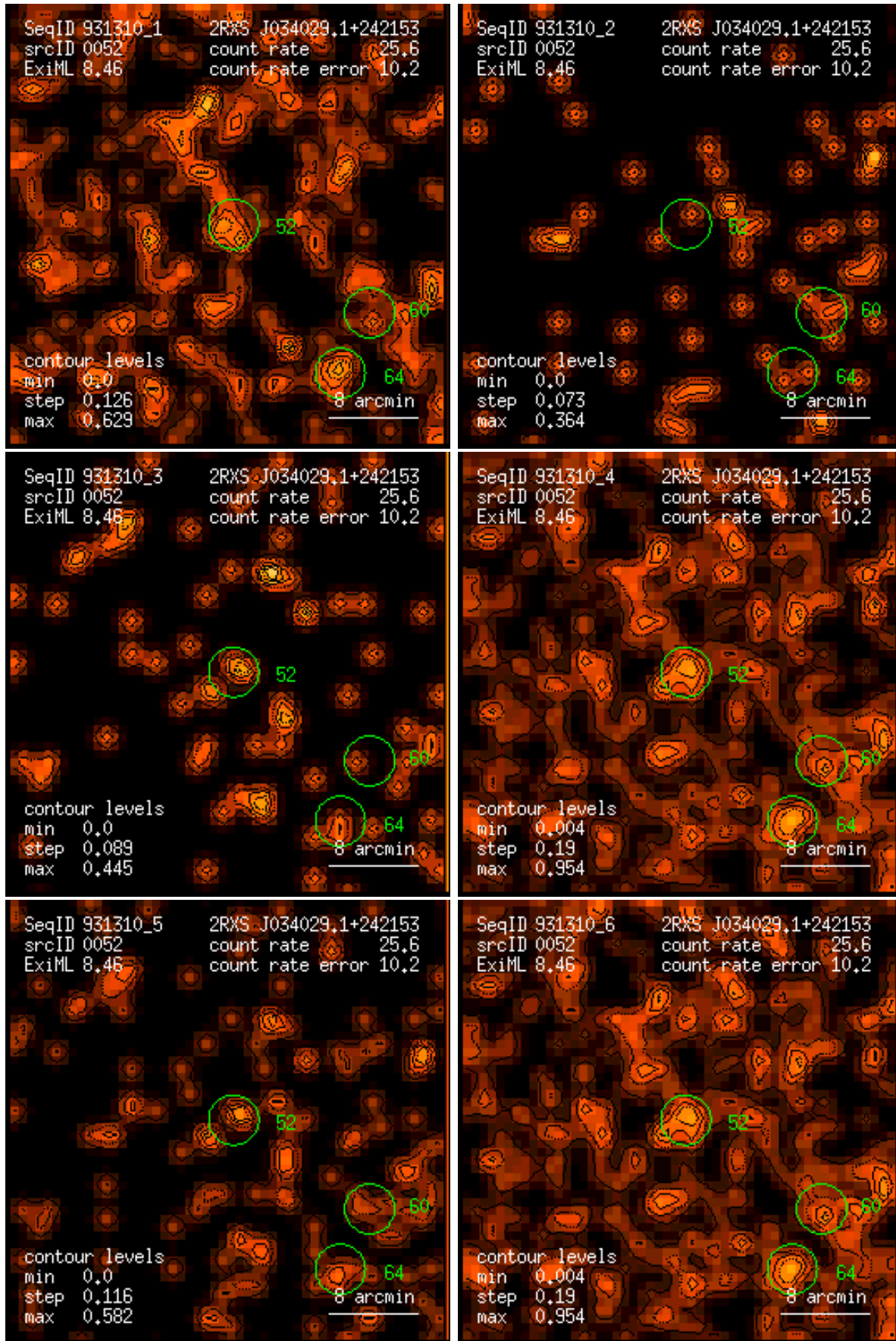
Figure 52: RASS 931310: detection 0052: band rate images, Gaussian filter: (1) PSPC channels 11 – 41, (2) 52 – 90, (3) 91 – 201, (4) 11 – 235, (5) 52 – 201, (6) 11 – 201. Broad band rates in counts/ks. Band rate contour levels in counts/ks/arcmin 2 .
