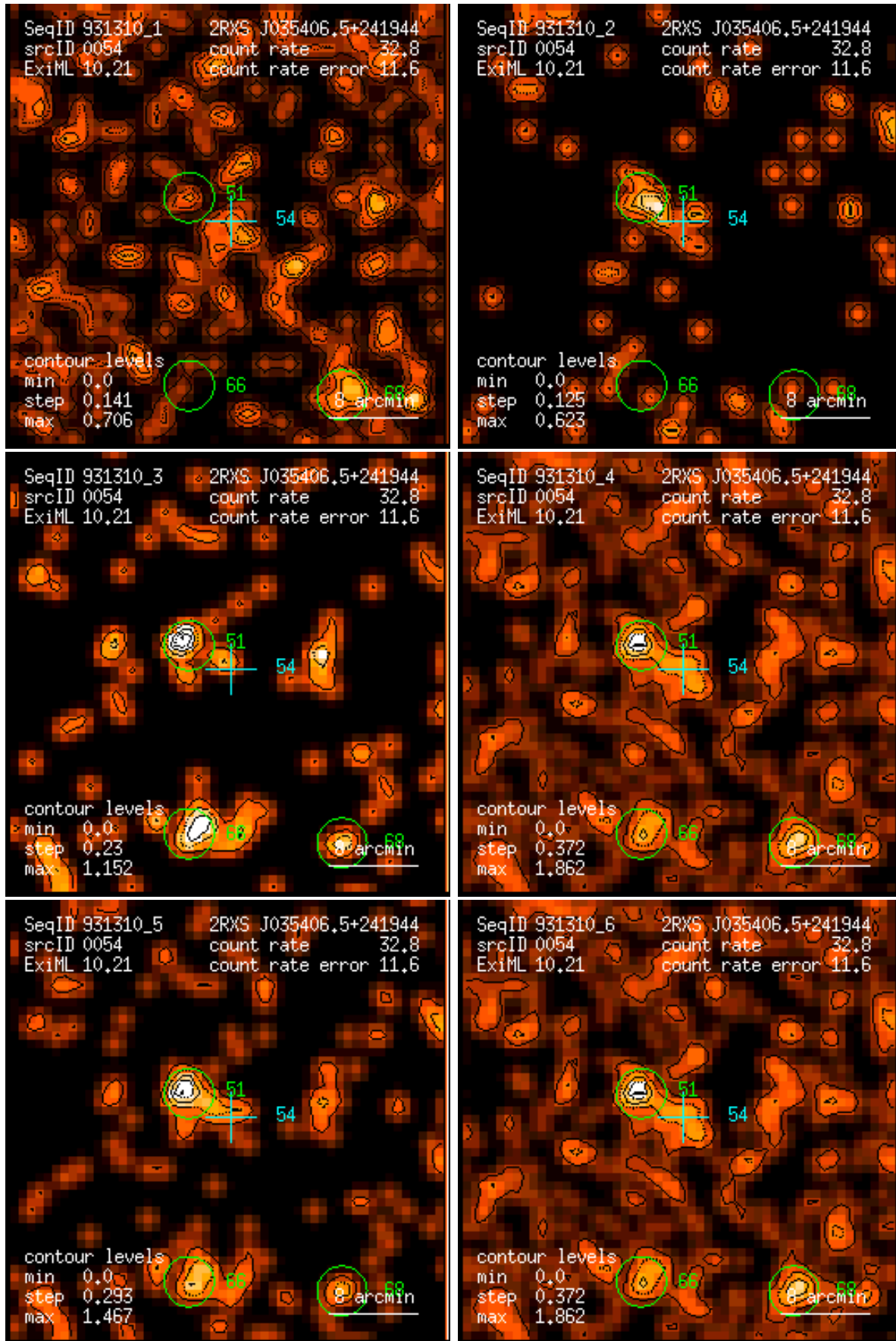
Figure 54: RASS 931310: detection 0054: band rate images, Gaussian filter: (1) PSPC channels 11 – 41, (2) 52 – 90, (3) 91 – 201, (4) 11 – 235, (5) 52 – 201, (6) 11 – 201. Broad band rates in counts/ks. Band rate contour levels in counts/ks/arcmin 2 .
