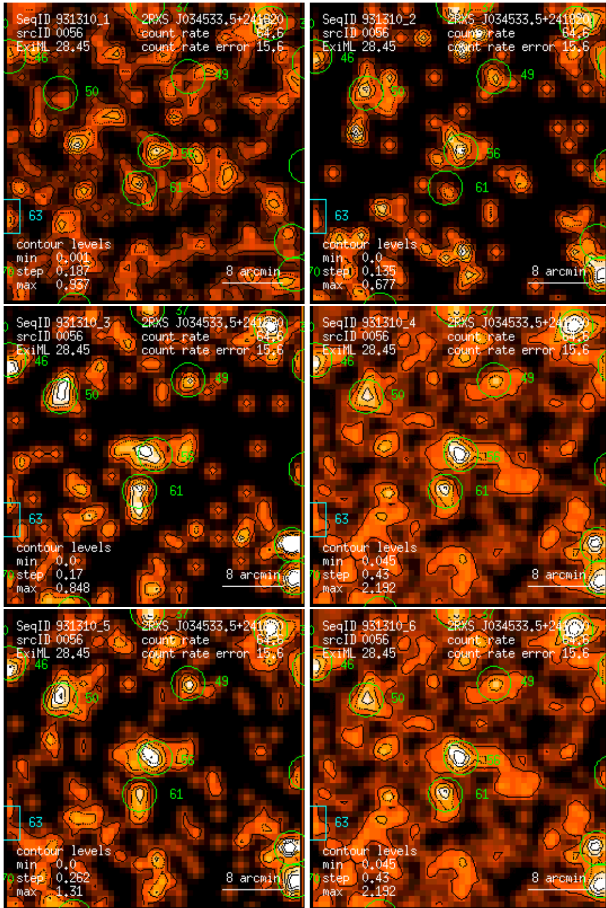
Figure 56: RASS 931310: detection 0056: band rate images, Gaussian filter: (1) PSPC channels 11 – 41, (2) 52 – 90, (3) 91 – 201, (4) 11 – 235, (5) 52 – 201, (6) 11 – 201. Broad band rates in counts/ks. Band rate contour levels in counts/ks/arcmin 2 .
