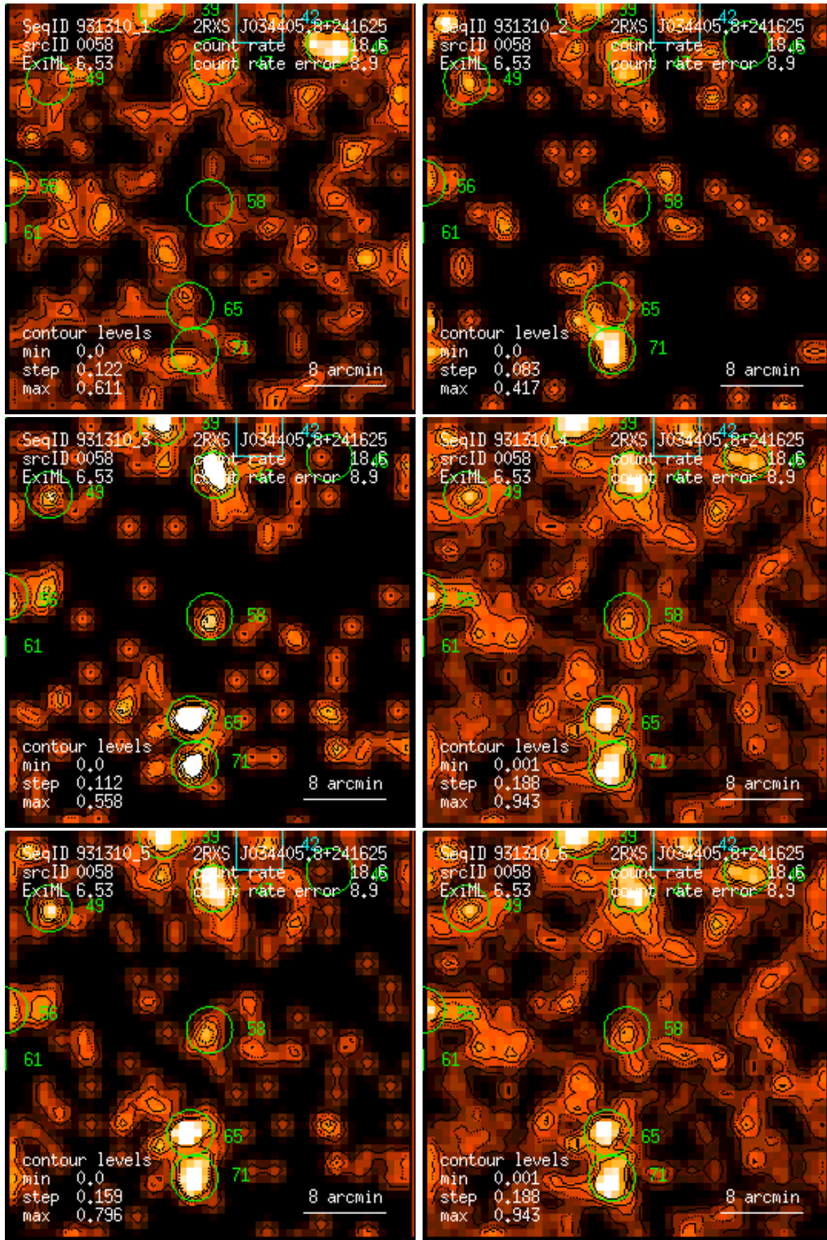
Figure 58: RASS 931310: detection 0058: band rate images, Gaussian filter: (1) PSPC channels 11 – 41, (2) 52 – 90, (3) 91 – 201, (4) 11 – 235, (5) 52 – 201, (6) 11 – 201. Broad band rates in counts/ks. Band rate contour levels in counts/ks/arcmin 2 .
