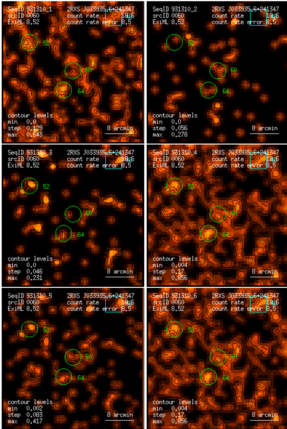
Figure 60: RASS 931310: detection 0060: band rate images, Gaussian filter: (1) PSPC channels 11 – 41, (2) 52 – 90, (3) 91 – 201, (4) 11 – 235, (5) 52 – 201, (6) 11 – 201. Broad band rates in counts/ks. Band rate contour levels in counts/ks/arcmin 2 .
