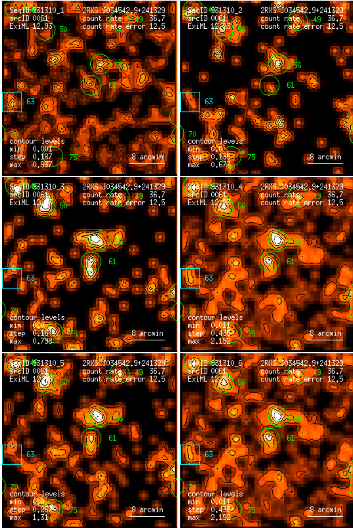
Figure 61: RASS 931310: detection 0061: band rate images, Gaussian filter: (1) PSPC channels 11 – 41, (2) 52 – 90, (3) 91 – 201, (4) 11 – 235, (5) 52 – 201, (6) 11 – 201. Broad band rates in counts/ks. Band rate contour levels in counts/ks/arcmin 2 .
