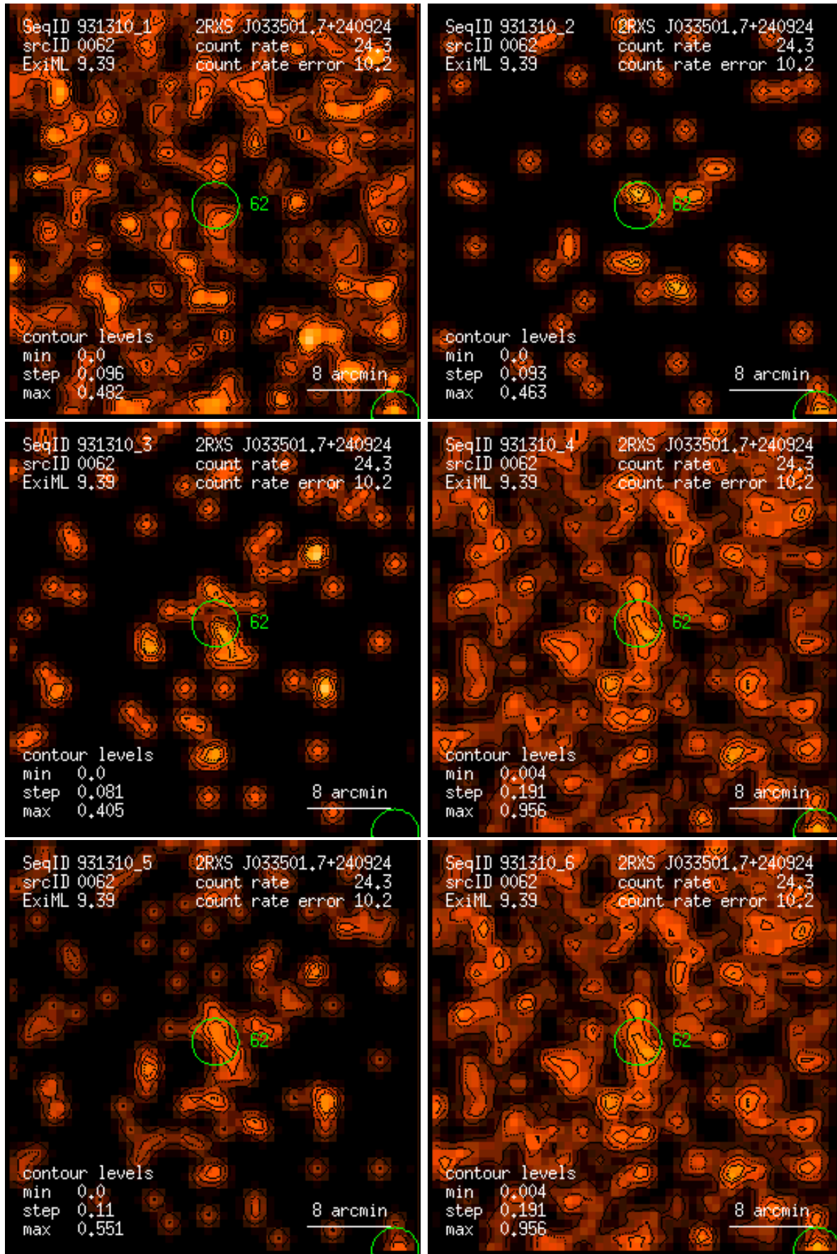
Figure 62: RASS 931310: detection 0062: band rate images, Gaussian filter: (1) PSPC channels 11 – 41, (2) 52 – 90, (3) 91 – 201, (4) 11 – 235, (5) 52 – 201, (6) 11 – 201. Broad band rates in counts/ks. Band rate contour levels in counts/ks/arcmin 2 .
