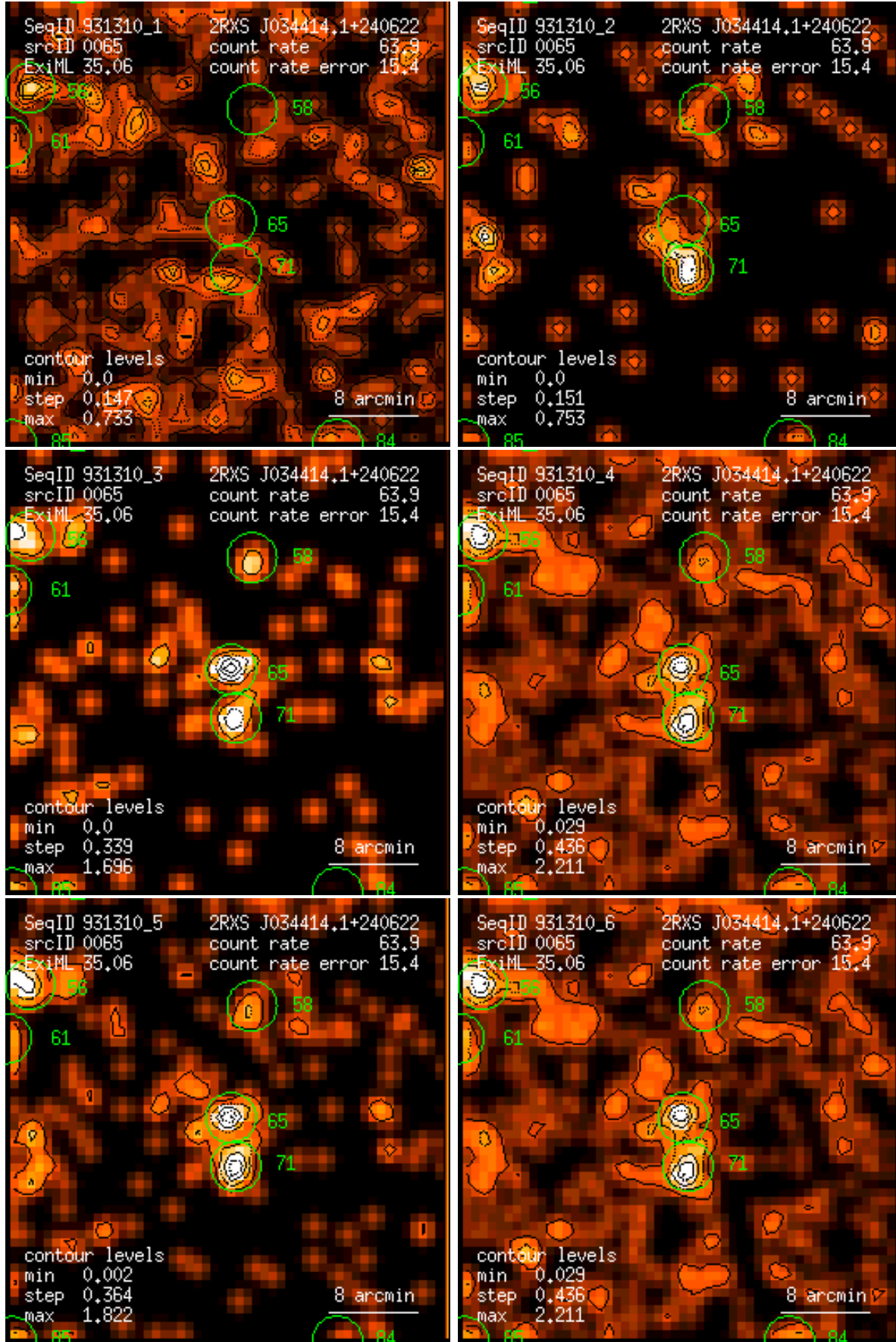
Figure 65: RASS 931310: detection 0065: band rate images, Gaussian filter: (1) PSPC channels 11 – 41, (2) 52 – 90, (3) 91 – 201, (4) 11 – 235, (5) 52 – 201, (6) 11 – 201. Broad band rates in counts/ks. Band rate contour levels in counts/ks/arcmin 2 .
