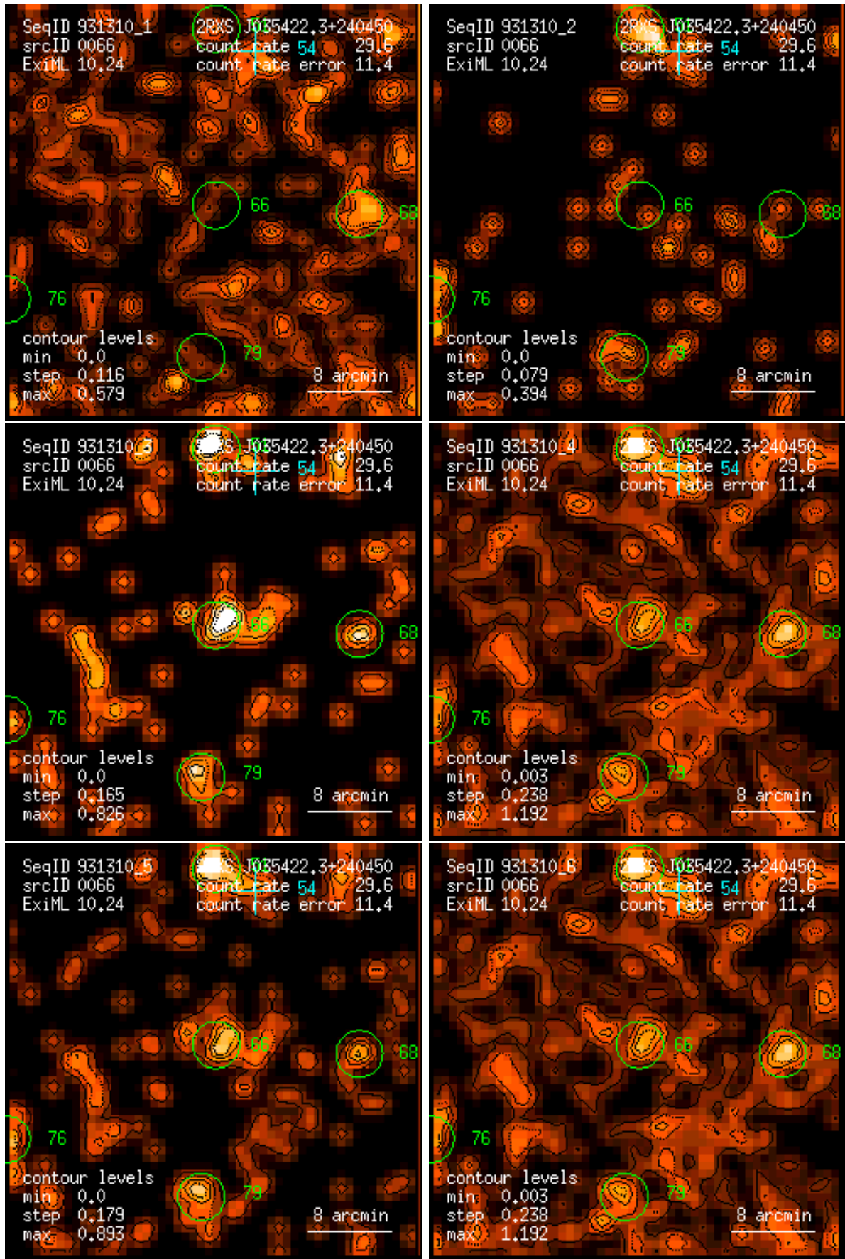
Figure 66: RASS 931310: detection 0066: band rate images, Gaussian filter: (1) PSPC channels 11 – 41, (2) 52 – 90, (3) 91 – 201, (4) 11 – 235, (5) 52 – 201, (6) 11 – 201. Broad band rates in counts/ks. Band rate contour levels in counts/ks/arcmin 2 .
