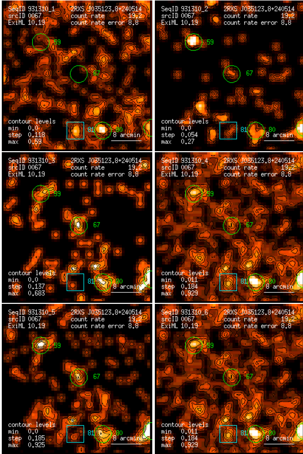
Figure 67: RASS 931310: detection 0067: band rate images, Gaussian filter: (1) PSPC channels 11 – 41, (2) 52 – 90, (3) 91 – 201, (4) 11 – 235, (5) 52 – 201, (6) 11 – 201. Broad band rates in counts/ks. Band rate contour levels in counts/ks/arcmin 2 .
