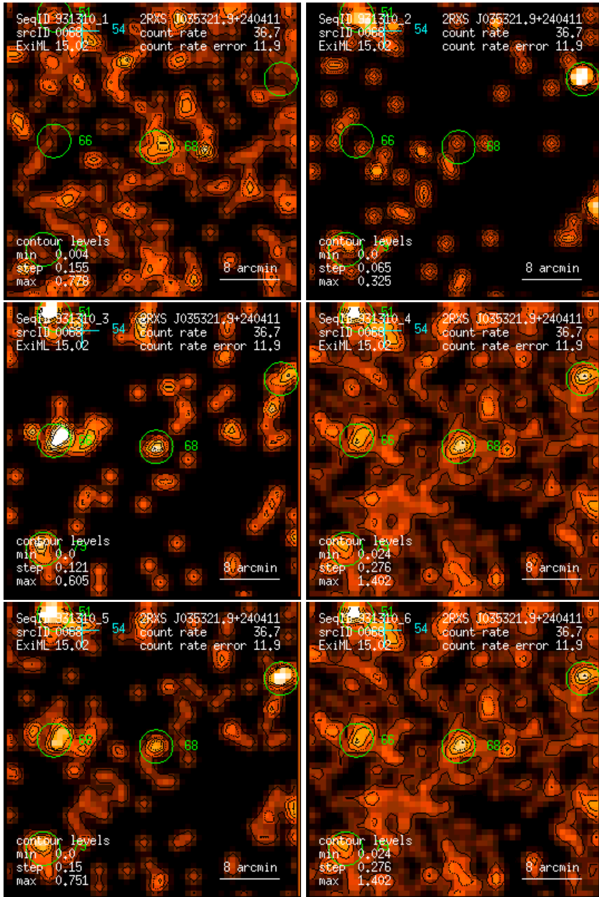
Figure 68: RASS 931310: detection 0068: band rate images, Gaussian filter: (1) PSPC channels 11 – 41, (2) 52 – 90, (3) 91 – 201, (4) 11 – 235, (5) 52 – 201, (6) 11 – 201. Broad band rates in counts/ks. Band rate contour levels in counts/ks/arcmin 2 .
