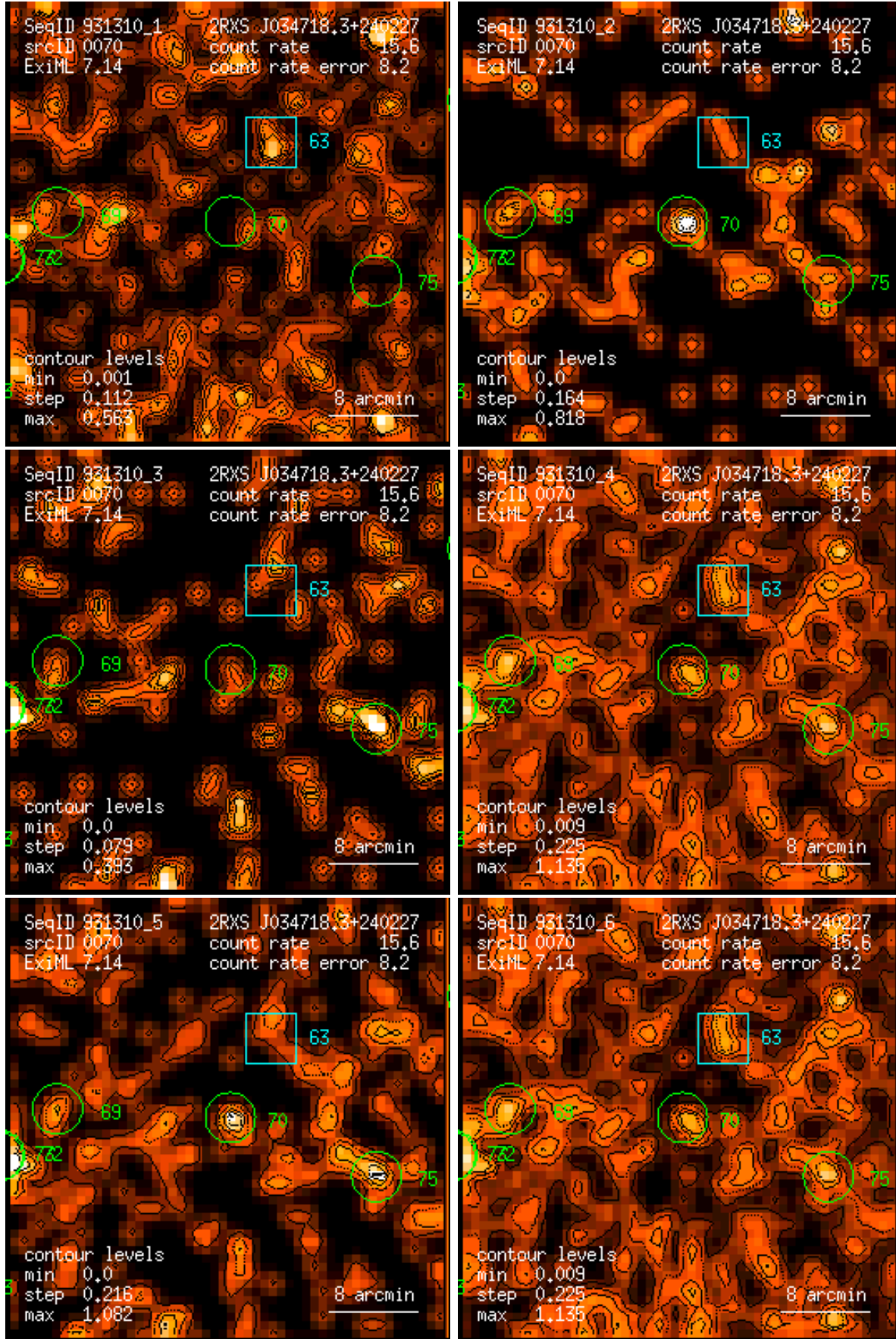
Figure 70: RASS 931310: detection 0070: band rate images, Gaussian filter: (1) PSPC channels 11 – 41, (2) 52 – 90, (3) 91 – 201, (4) 11 – 235, (5) 52 – 201, (6) 11 – 201. Broad band rates in counts/ks. Band rate contour levels in counts/ks/arcmin 2 .
