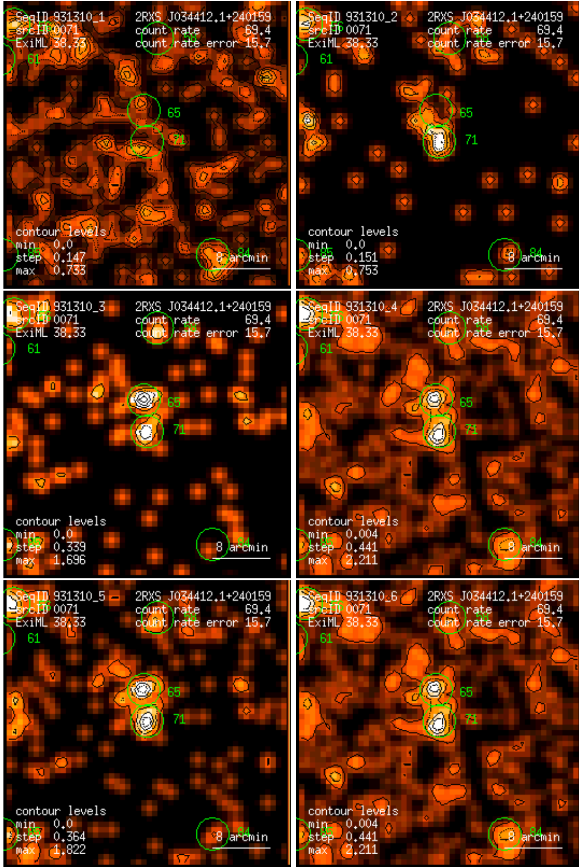
Figure 71: RASS 931310: detection 0071: band rate images, Gaussian filter: (1) PSPC channels 11 – 41, (2) 52 – 90, (3) 91 – 201, (4) 11 – 235, (5) 52 – 201, (6) 11 – 201. Broad band rates in counts/ks. Band rate contour levels in counts/ks/arcmin 2 .
