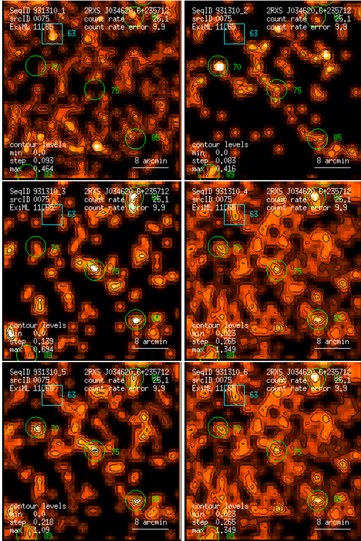
Figure 75: RASS 931310: detection 0075: band rate images, Gaussian filter: (1) PSPC channels 11 – 41, (2) 52 – 90, (3) 91 – 201, (4) 11 – 235, (5) 52 – 201, (6) 11 – 201. Broad band rates in counts/ks. Band rate contour levels in counts/ks/arcmin 2 .
