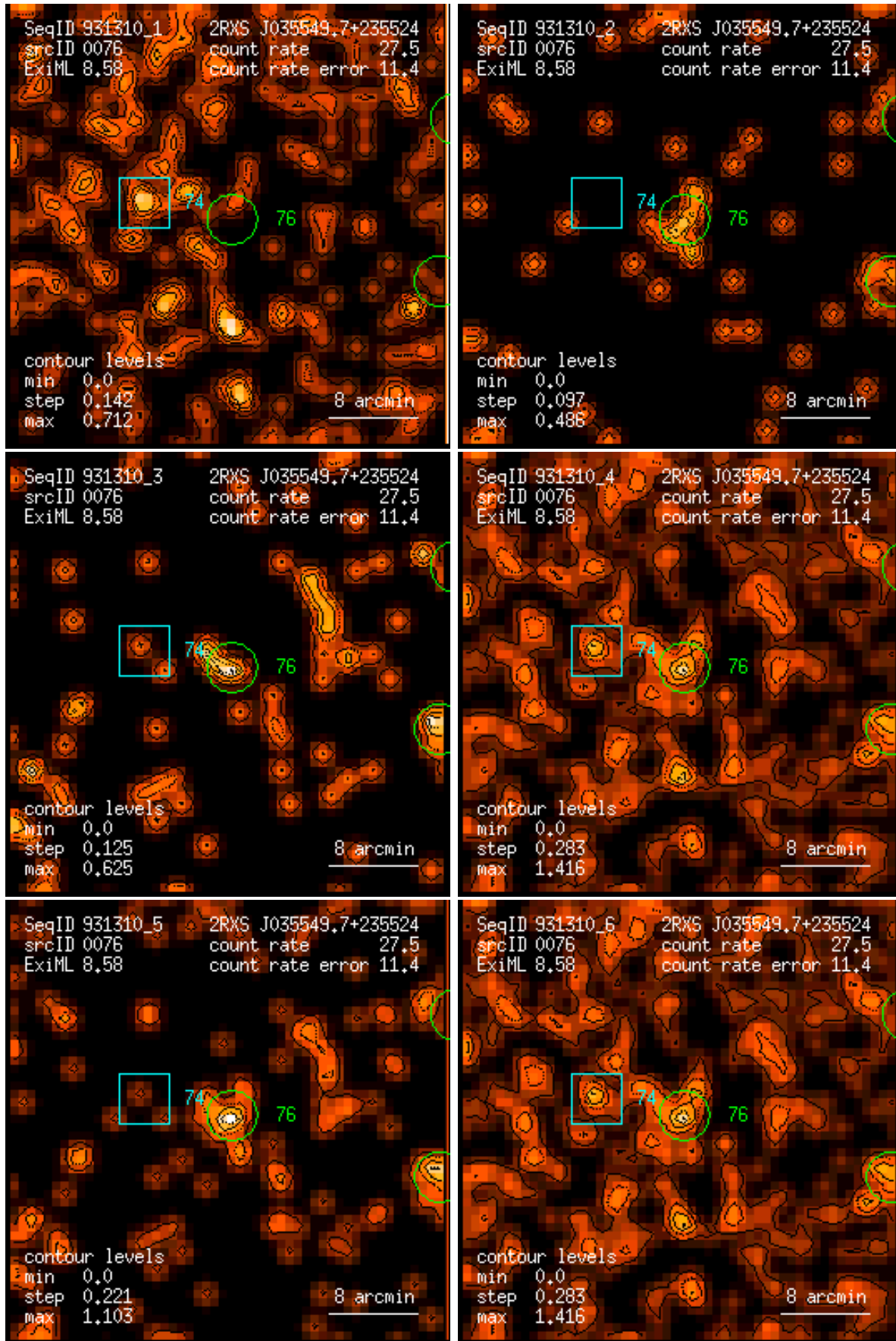
Figure 76: RASS 931310: detection 0076: band rate images, Gaussian filter: (1) PSPC channels 11 – 41, (2) 52 – 90, (3) 91 – 201, (4) 11 – 235, (5) 52 – 201, (6) 11 – 201. Broad band rates in counts/ks. Band rate contour levels in counts/ks/arcmin 2 .
