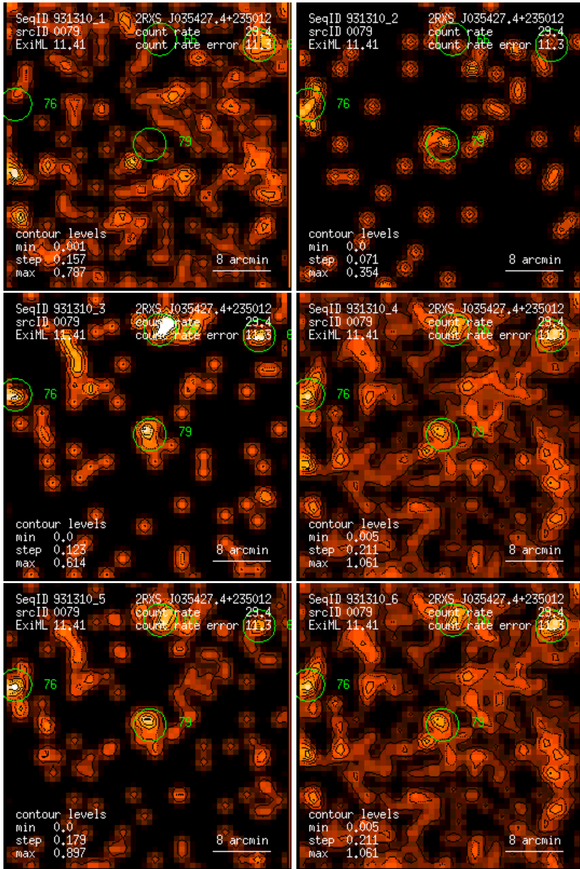
Figure 79: RASS 931310: detection 0079: band rate images, Gaussian filter: (1) PSPC channels 11 – 41, (2) 52 – 90, (3) 91 – 201, (4) 11 – 235, (5) 52 – 201, (6) 11 – 201. Broad band rates in counts/ks. Band rate contour levels in counts/ks/arcmin 2 .
