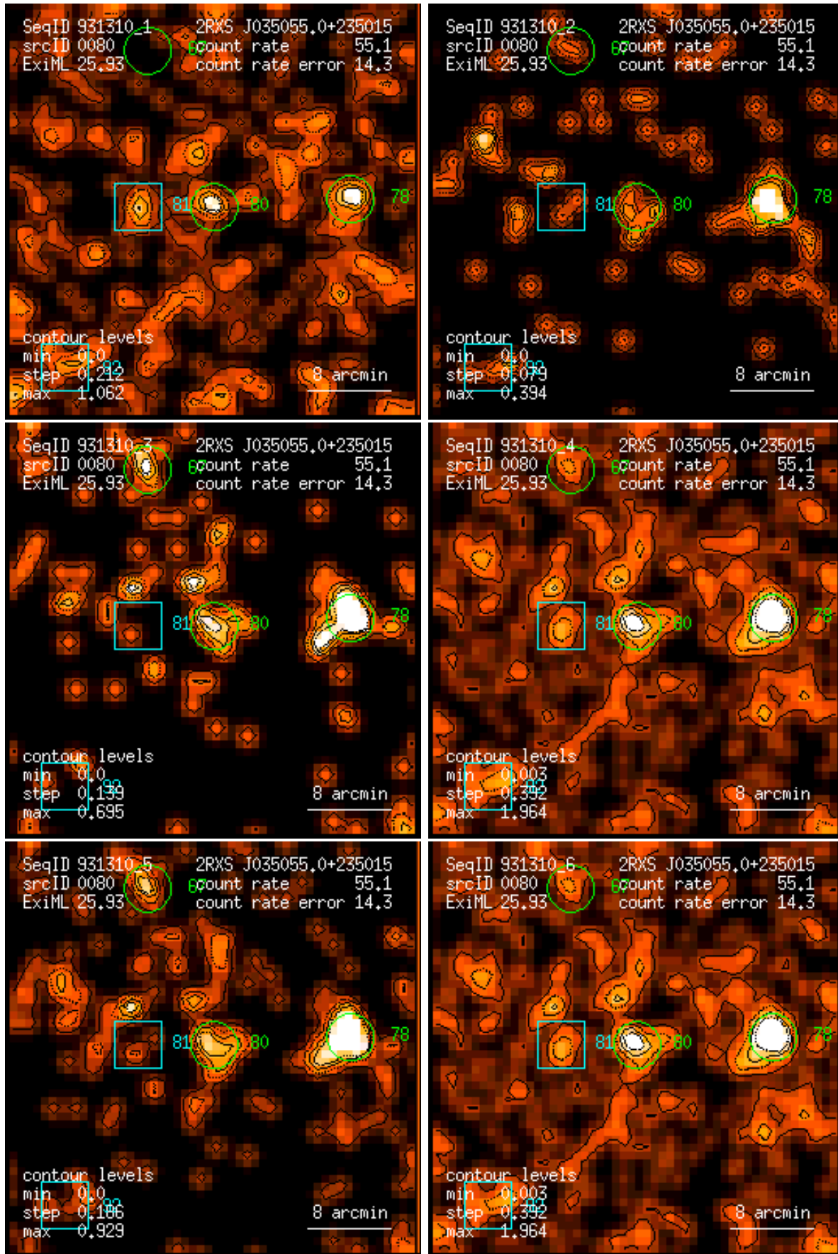
Figure 80: RASS 931310: detection 0080: band rate images, Gaussian filter: (1) PSPC channels 11 – 41, (2) 52 – 90, (3) 91 – 201, (4) 11 – 235, (5) 52 – 201, (6) 11 – 201. Broad band rates in counts/ks. Band rate contour levels in counts/ks/arcmin 2 .
