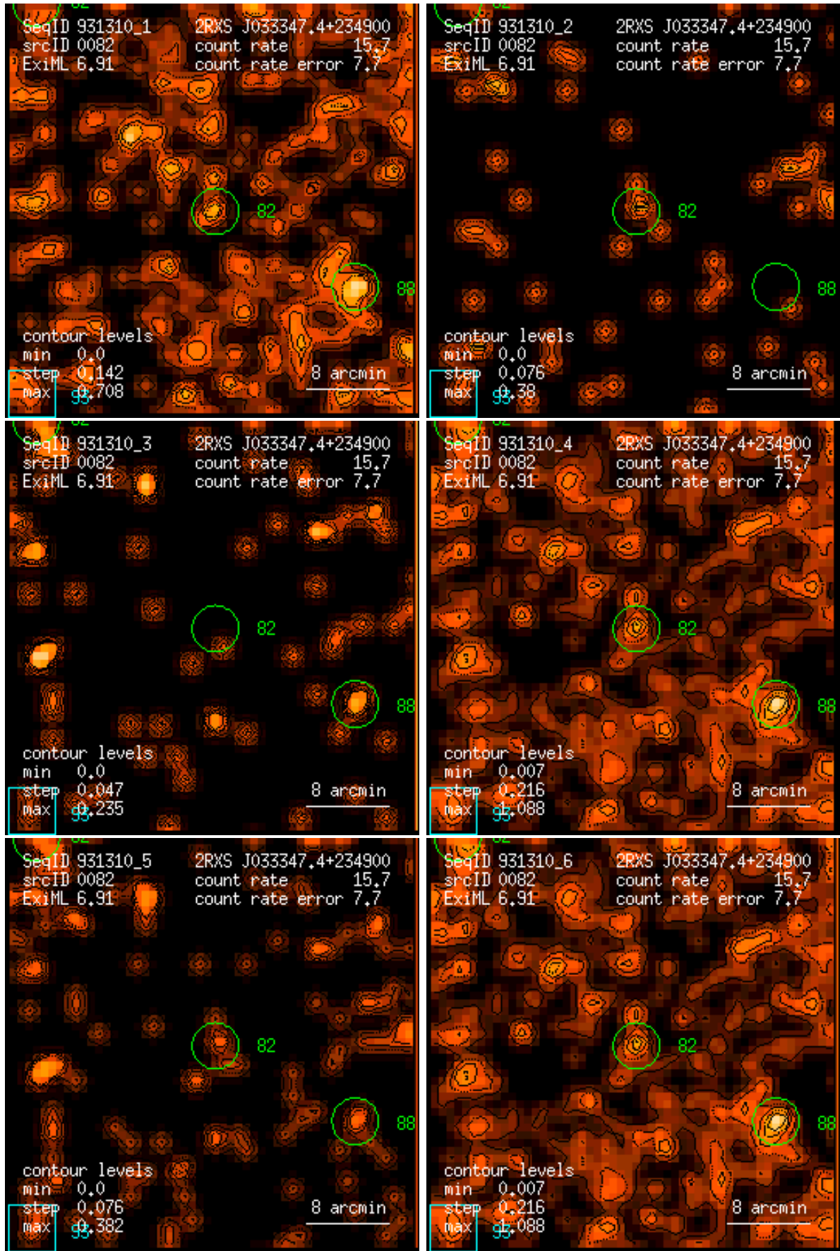
Figure 82: RASS 931310: detection 0082: band rate images, Gaussian filter: (1) PSPC channels 11 – 41, (2) 52 – 90, (3) 91 – 201, (4) 11 – 235, (5) 52 – 201, (6) 11 – 201. Broad band rates in counts/ks. Band rate contour levels in counts/ks/arcmin 2 .
