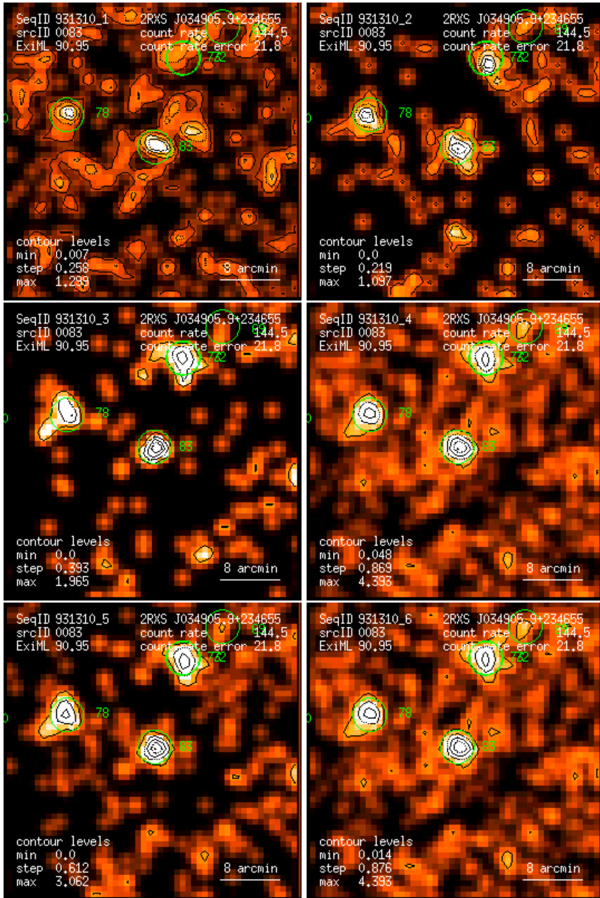
Figure 83: RASS 931310: detection 0083: band rate images, Gaussian filter: (1) PSPC channels 11 – 41, (2) 52 – 90, (3) 91 – 201, (4) 11 – 235, (5) 52 – 201, (6) 11 – 201. Broad band rates in counts/ks. Band rate contour levels in counts/ks/arcmin 2 .
