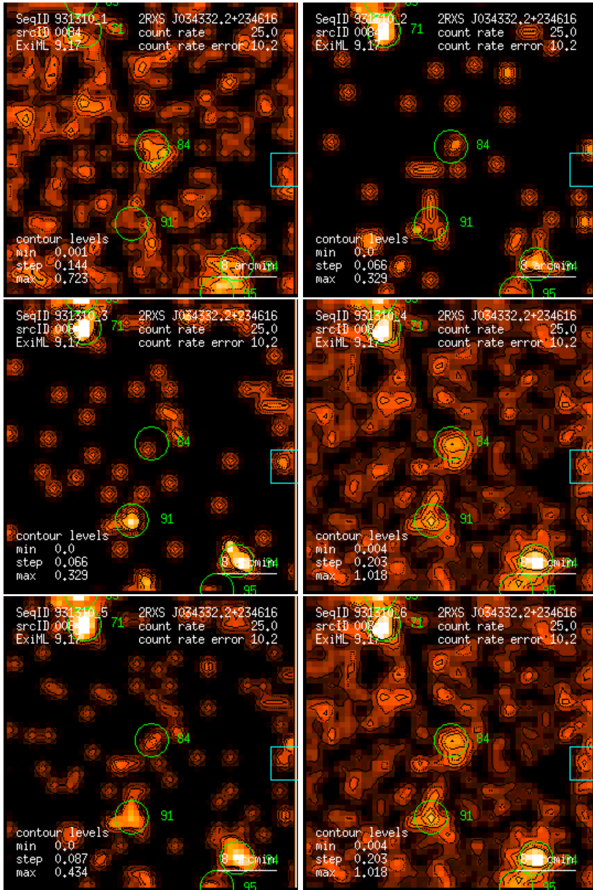
Figure 84: RASS 931310: detection 0084: band rate images, Gaussian filter: (1) PSPC channels 11 – 41, (2) 52 – 90, (3) 91 – 201, (4) 11 – 235, (5) 52 – 201, (6) 11 – 201. Broad band rates in counts/ks. Band rate contour levels in counts/ks/arcmin 2 .
