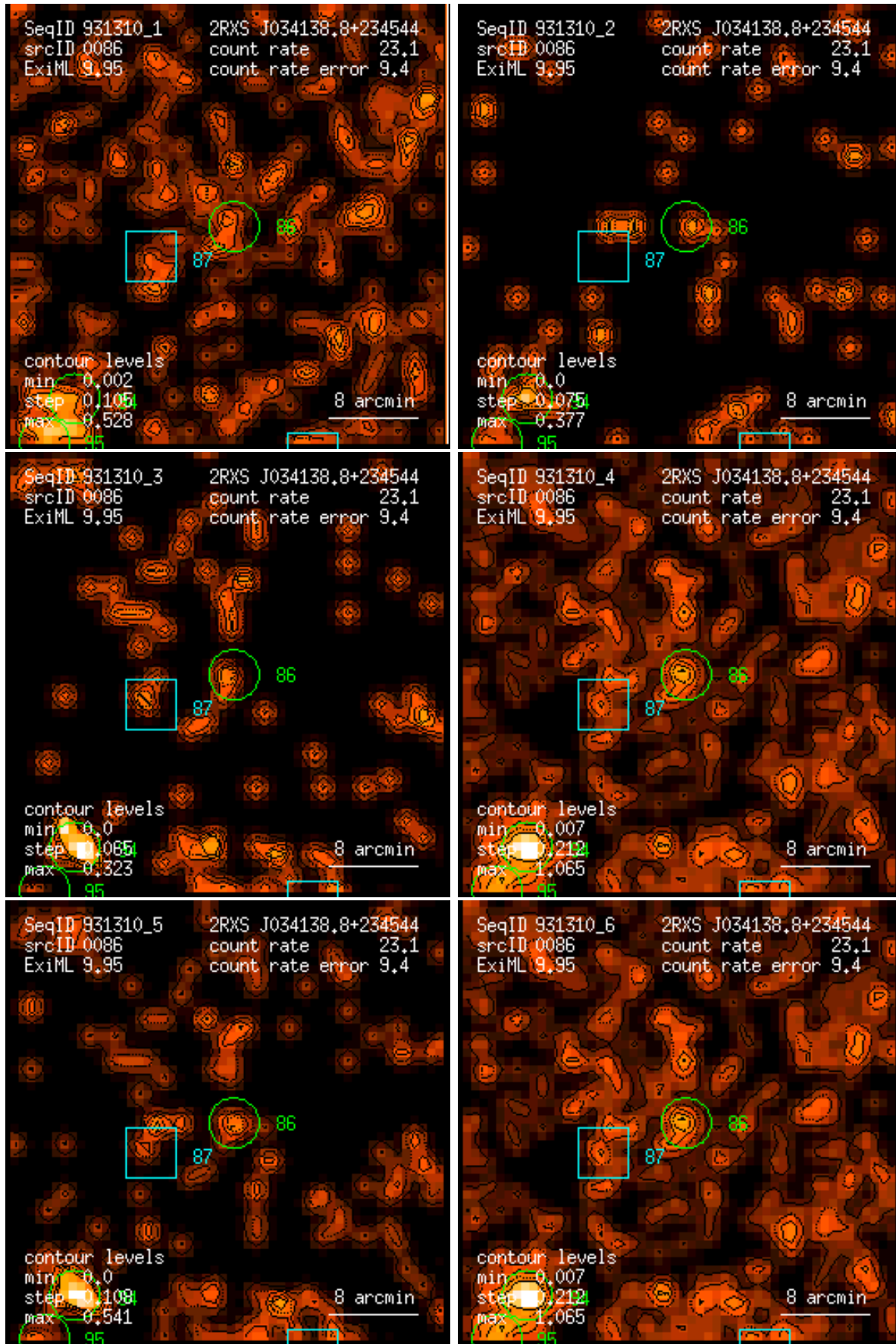
Figure 86: RASS 931310: detection 0086: band rate images, Gaussian filter: (1) PSPC channels 11 – 41, (2) 52 – 90, (3) 91 – 201, (4) 11 – 235, (5) 52 – 201, (6) 11 – 201. Broad band rates in counts/ks. Band rate contour levels in counts/ks/arcmin 2 .
