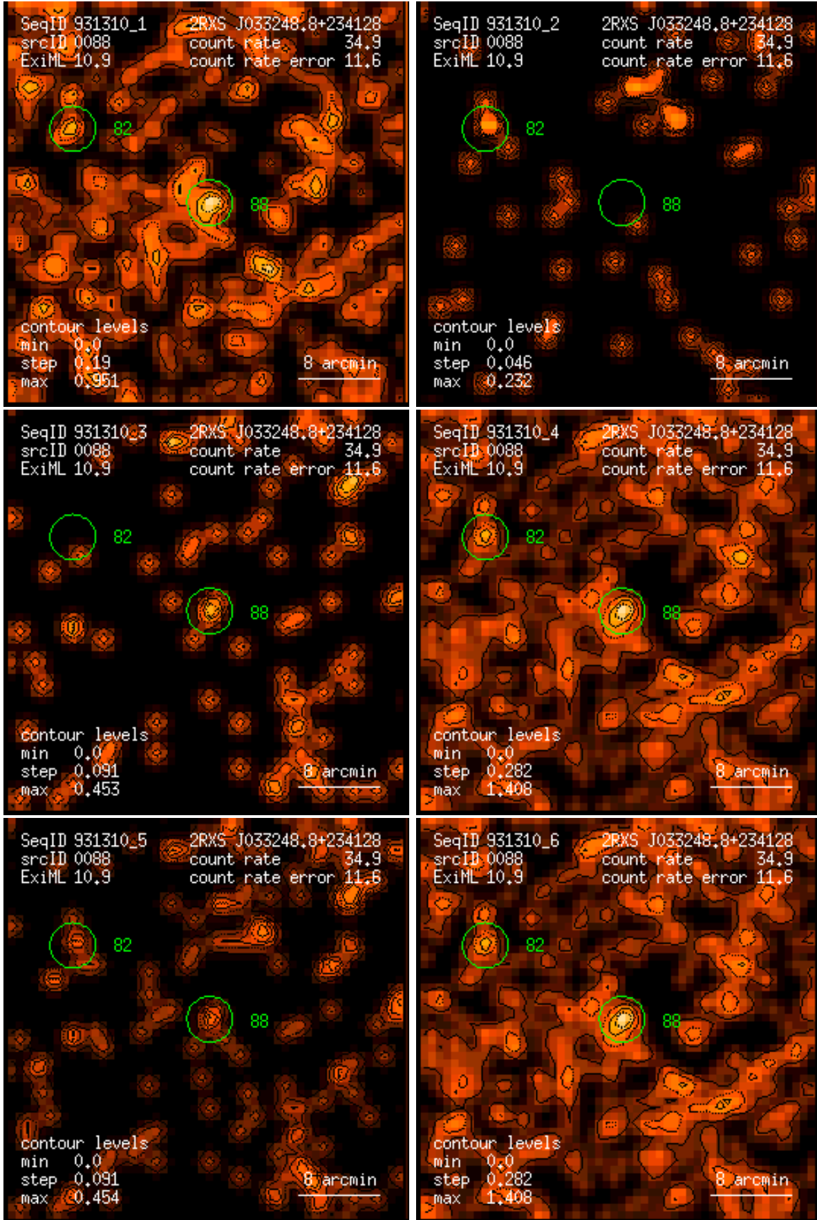
Figure 88: RASS 931310: detection 0088: band rate images, Gaussian filter: (1) PSPC channels 11 – 41, (2) 52 – 90, (3) 91 – 201, (4) 11 – 235, (5) 52 – 201, (6) 11 – 201. Broad band rates in counts/ks. Band rate contour levels in counts/ks/arcmin 2 .
