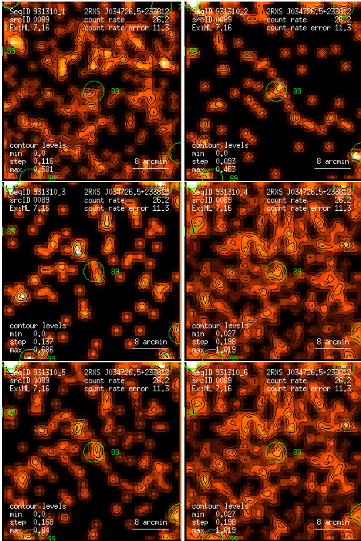
Figure 89: RASS 931310: detection 0089: band rate images, Gaussian filter: (1) PSPC channels 11 – 41, (2) 52 – 90, (3) 91 – 201, (4) 11 – 235, (5) 52 – 201, (6) 11 – 201. Broad band rates in counts/ks. Band rate contour levels in counts/ks/arcmin 2 .
