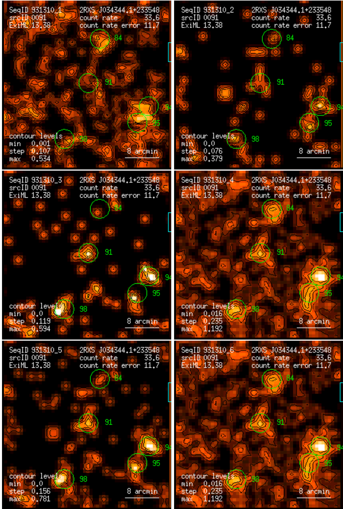
Figure 91: RASS 931310: detection 0091: band rate images, Gaussian filter: (1) PSPC channels 11 – 41, (2) 52 – 90, (3) 91 – 201, (4) 11 – 235, (5) 52 – 201, (6) 11 – 201. Broad band rates in counts/ks. Band rate contour levels in counts/ks/arcmin 2 .
