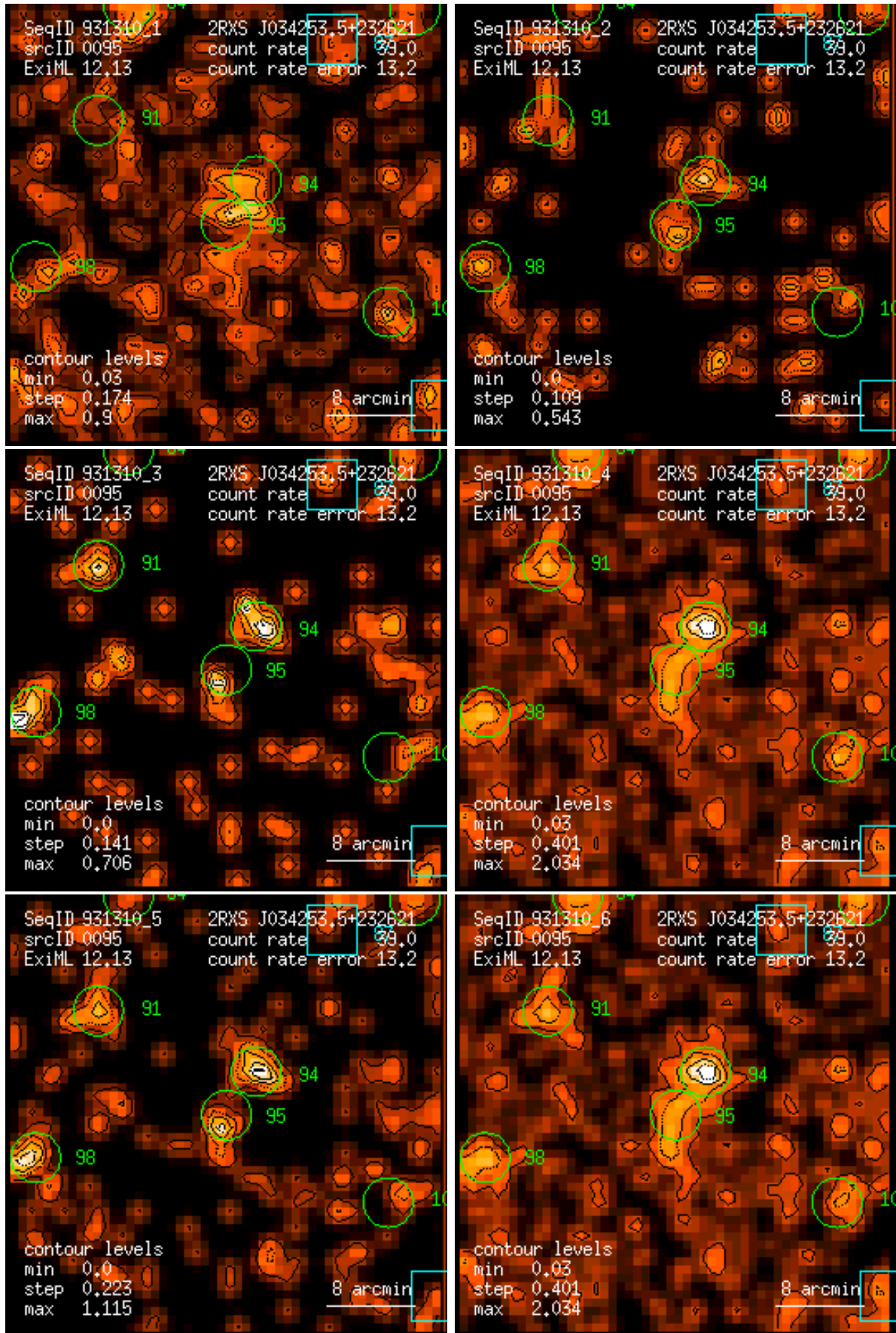
Figure 95: RASS 931310: detection 0095: band rate images, Gaussian filter: (1) PSPC channels 11 – 41, (2) 52 – 90, (3) 91 – 201, (4) 11 – 235, (5) 52 – 201, (6) 11 – 201. Broad band rates in counts/ks. Band rate contour levels in counts/ks/arcmin 2 .
