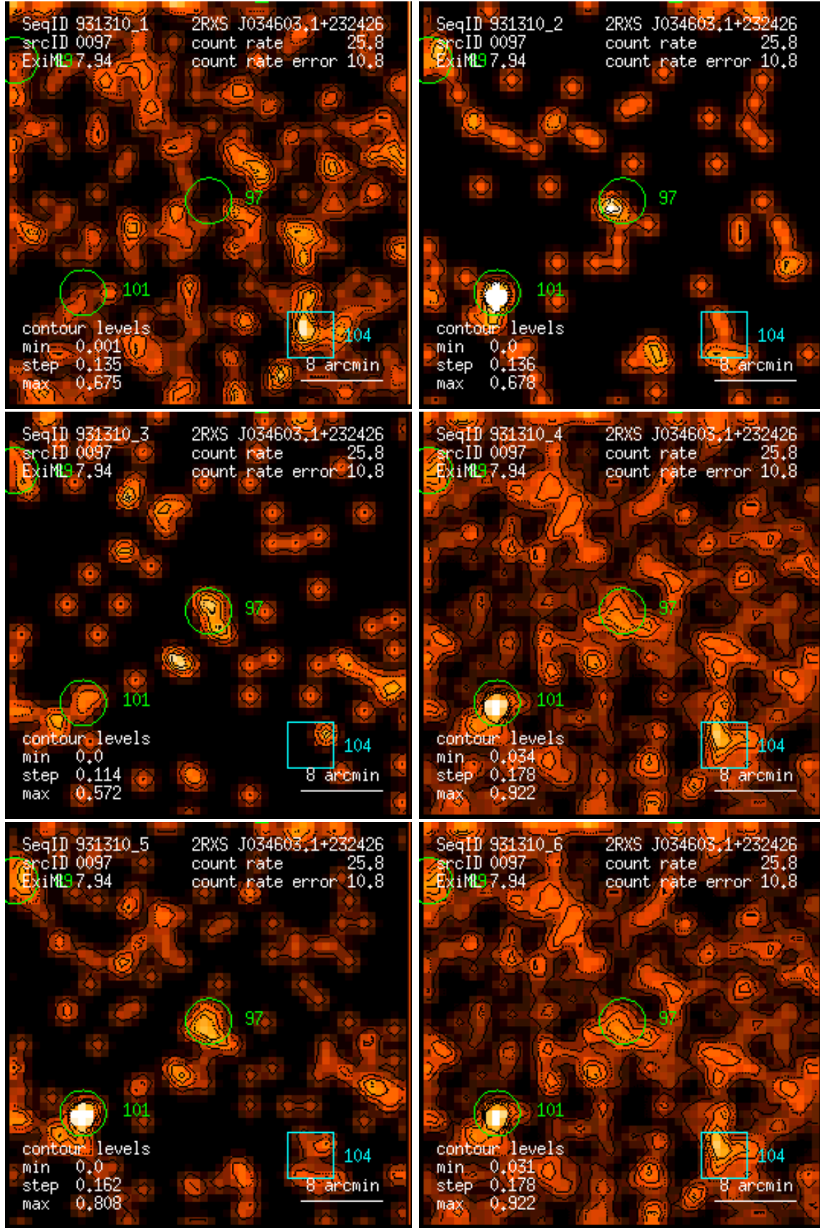
Figure 97: RASS 931310: detection 0097: band rate images, Gaussian filter: (1) PSPC channels 11 – 41, (2) 52 – 90, (3) 91 – 201, (4) 11 – 235, (5) 52 – 201, (6) 11 – 201. Broad band rates in counts/ks. Band rate contour levels in counts/ks/arcmin 2 .
