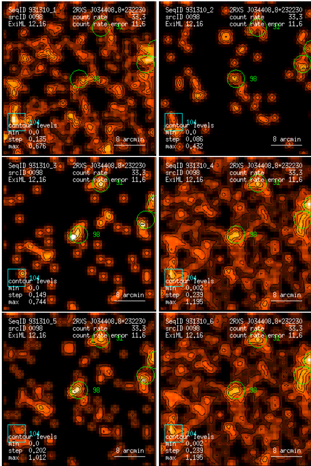
Figure 98: RASS 931310: detection 0098: band rate images, Gaussian filter: (1) PSPC channels 11 – 41, (2) 52 – 90, (3) 91 – 201, (4) 11 – 235, (5) 52 – 201, (6) 11 – 201. Broad band rates in counts/ks. Band rate contour levels in counts/ks/arcmin 2 .
