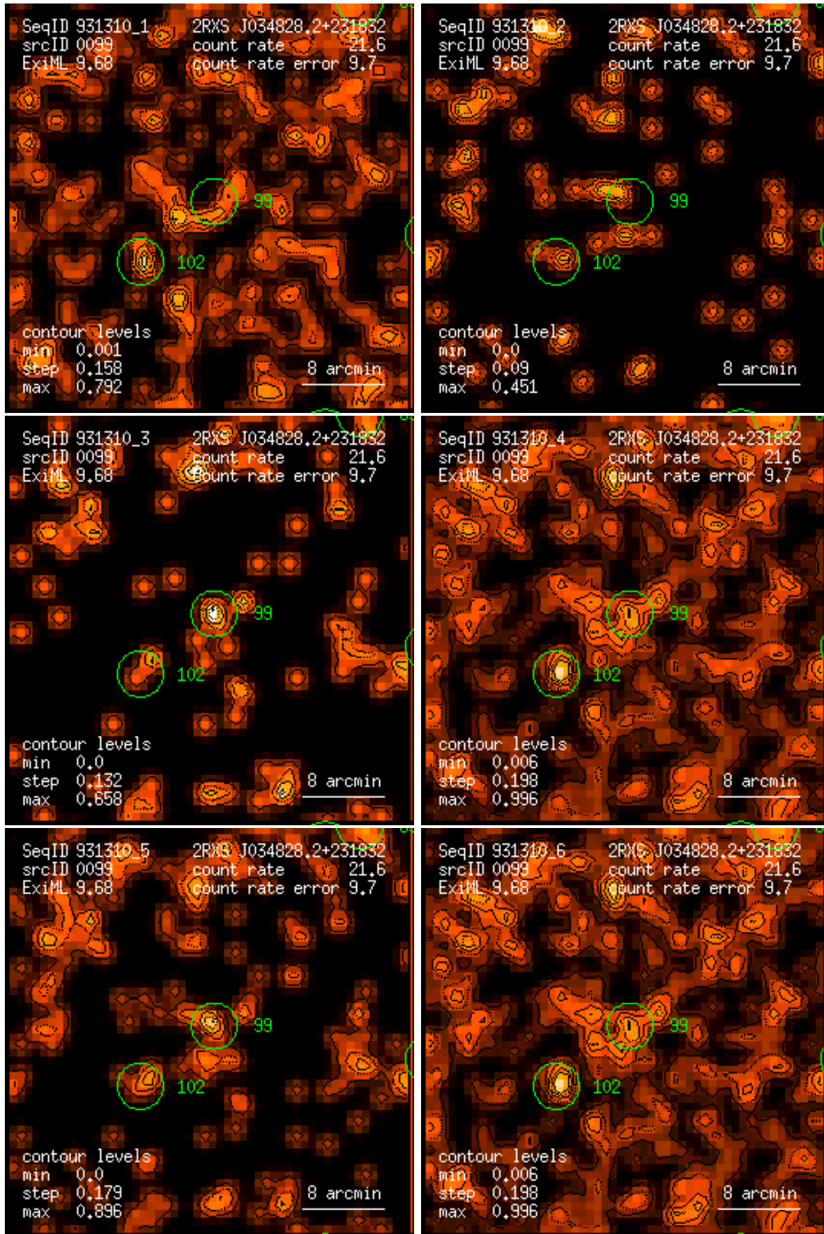
Figure 99: RASS 931310: detection 0099: band rate images, Gaussian filter: (1) PSPC channels 11 – 41, (2) 52 – 90, (3) 91 – 201, (4) 11 – 235, (5) 52 – 201, (6) 11 – 201. Broad band rates in counts/ks. Band rate contour levels in counts/ks/arcmin 2 .
