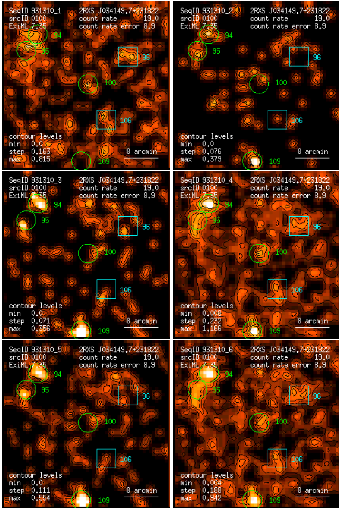
Figure 100: RASS 931310: detection 0100: band rate images, Gaussian filter: (1) PSPC channels 11 – 41, (2) 52 – 90, (3) 91 – 201, (4) 11 – 235, (5) 52 – 201, (6) 11 – 201. Broad band rates in counts/ks. Band rate contour levels in counts/ks/arcmin 2 .
