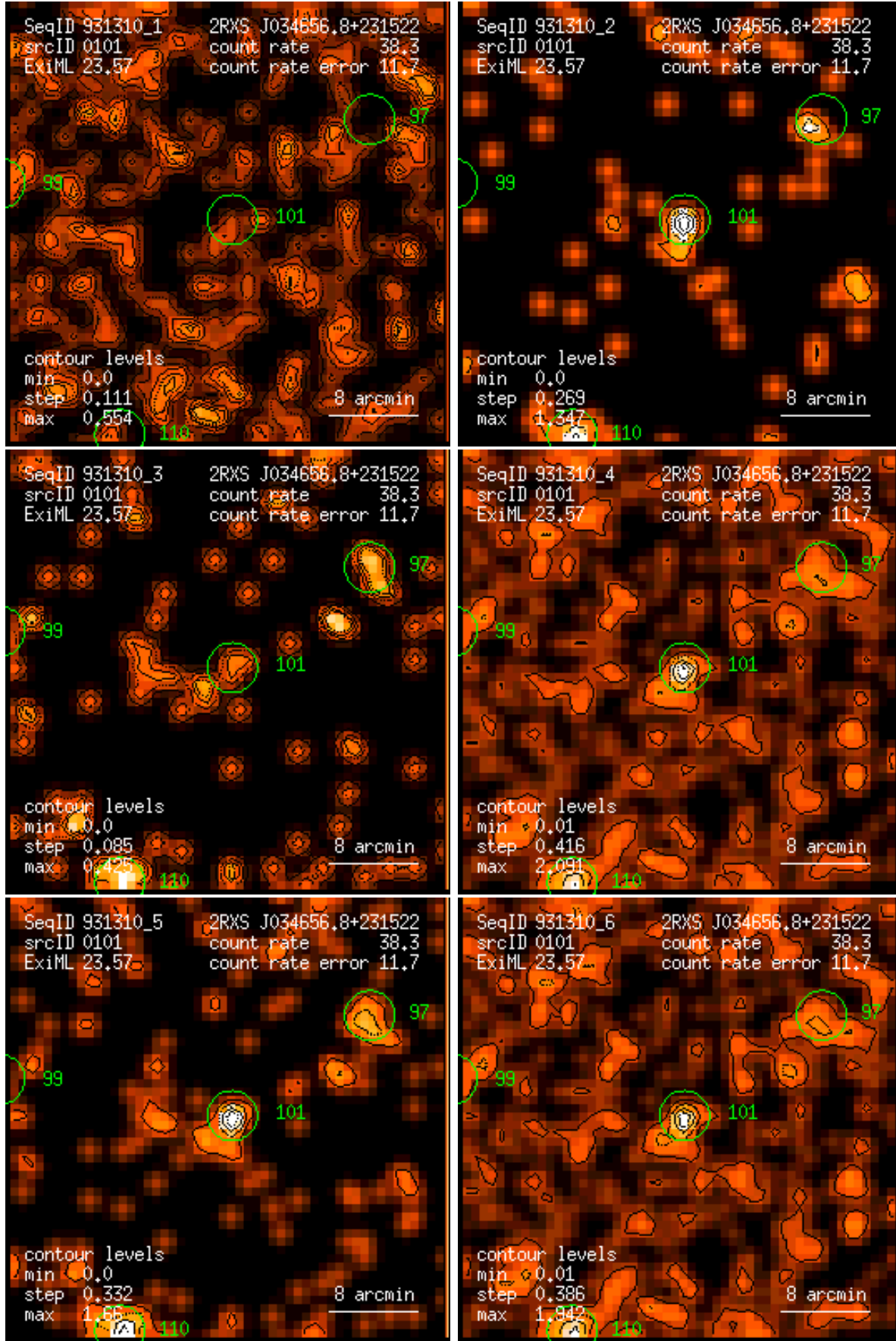
Figure 101: RASS 931310: detection 0101: band rate images, Gaussian filter: (1) PSPC channels 11 – 41, (2) 52 – 90, (3) 91 – 201, (4) 11 – 235, (5) 52 – 201, (6) 11 – 201. Broad band rates in counts/ks. Band rate contour levels in counts/ks/arcmin 2 .
