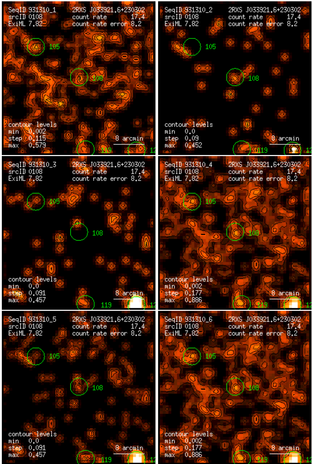
Figure 108: RASS 931310: detection 0108: band rate images, Gaussian filter: (1) PSPC channels 11 – 41, (2) 52 – 90, (3) 91 – 201, (4) 11 – 235, (5) 52 – 201, (6) 11 – 201. Broad band rates in counts/ks. Band rate contour levels in counts/ks/arcmin 2 .
