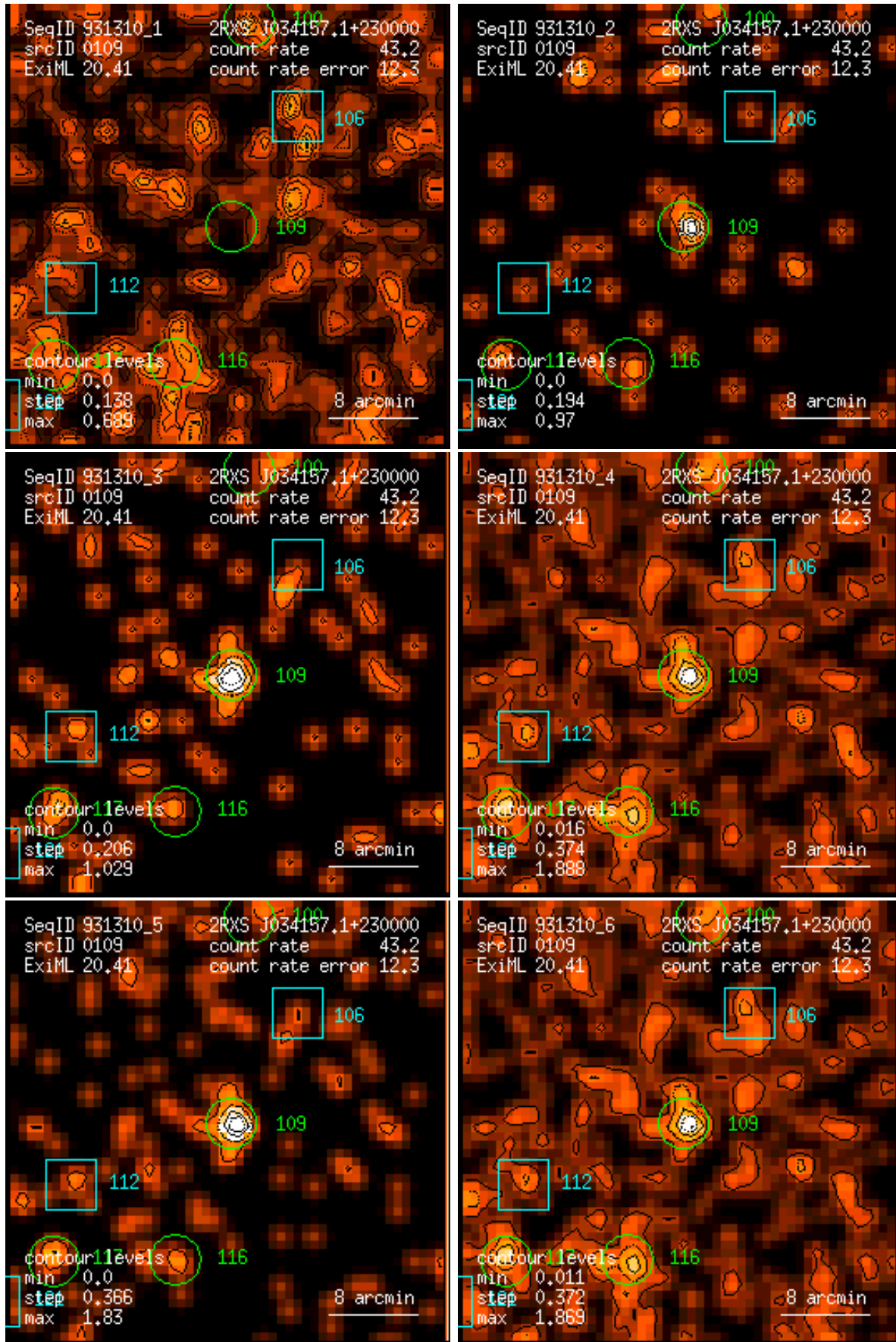
Figure 109: RASS 931310: detection 0109: band rate images, Gaussian filter: (1) PSPC channels 11 – 41, (2) 52 – 90, (3) 91 – 201, (4) 11 – 235, (5) 52 – 201, (6) 11 – 201. Broad band rates in counts/ks. Band rate contour levels in counts/ks/arcmin 2 .
