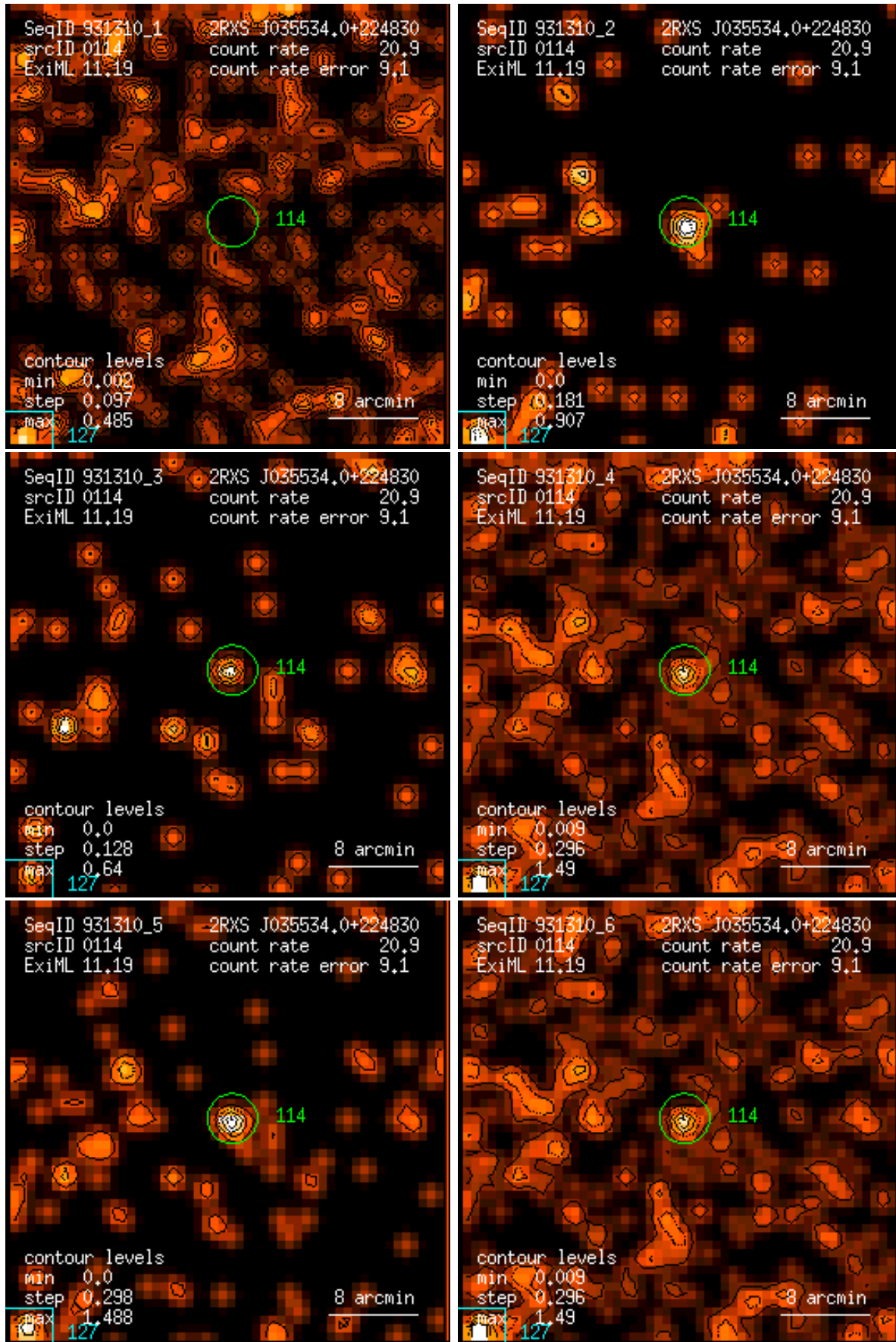
Figure 114: RASS 931310: detection 0114: band rate images, Gaussian filter: (1) PSPC channels 11 – 41, (2) 52 – 90, (3) 91 – 201, (4) 11 – 235, (5) 52 – 201, (6) 11 – 201. Broad band rates in counts/ks. Band rate contour levels in counts/ks/arcmin 2 .
