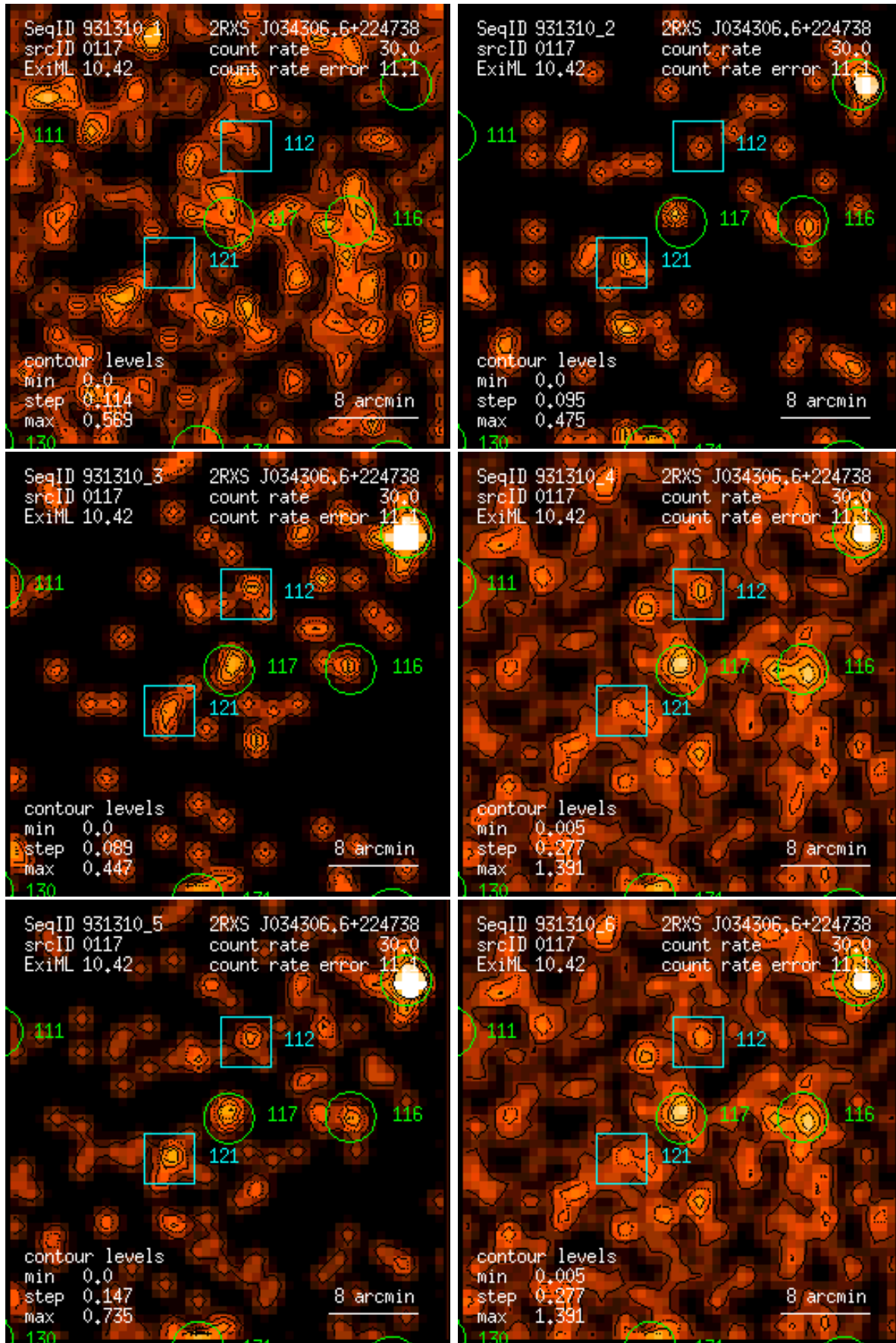
Figure 117: RASS 931310: detection 0117: band rate images, Gaussian filter: (1) PSPC channels 11 – 41, (2) 52 – 90, (3) 91 – 201, (4) 11 – 235, (5) 52 – 201, (6) 11 – 201. Broad band rates in counts/ks. Band rate contour levels in counts/ks/arcmin 2 .
