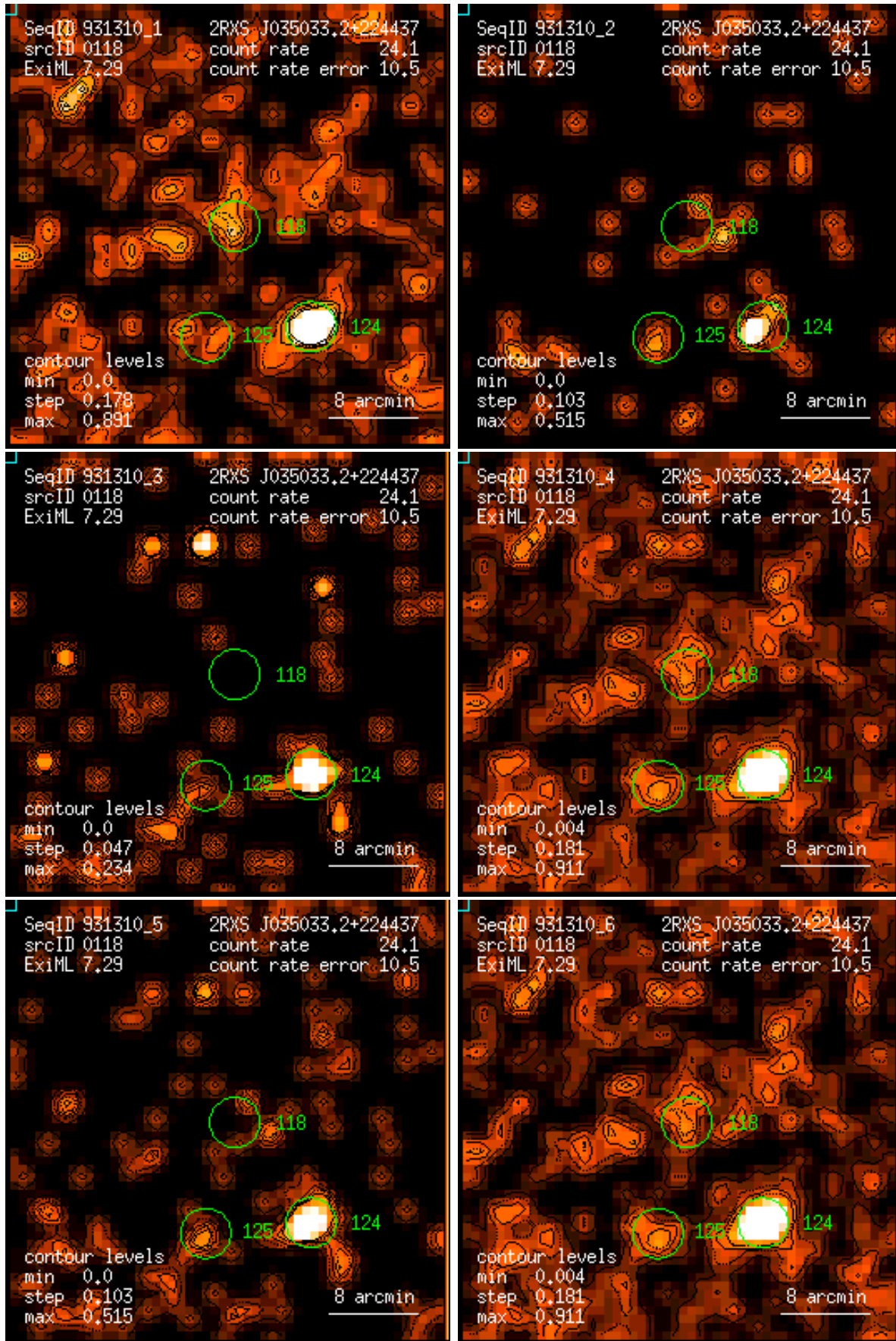
Figure 118: RASS 931310: detection 0118: band rate images, Gaussian filter: (1) PSPC channels 11 – 41, (2) 52 – 90, (3) 91 – 201, (4) 11 – 235, (5) 52 – 201, (6) 11 – 201. Broad band rates in counts/ks. Band rate contour levels in counts/ks/arcmin 2 .
