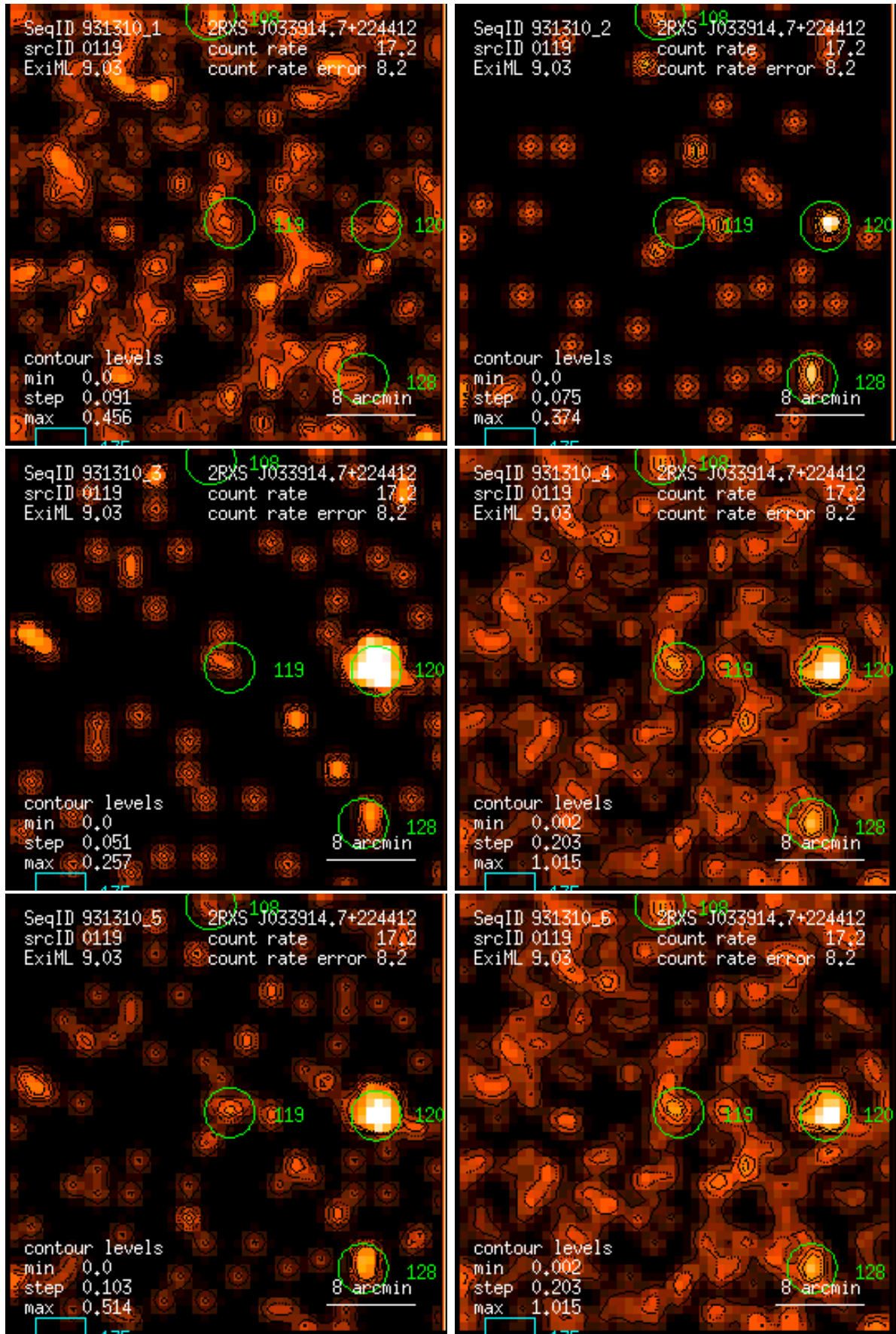
Figure 119: RASS 931310: detection 0119: band rate images, Gaussian filter: (1) PSPC channels 11 – 41, (2) 52 – 90, (3) 91 – 201, (4) 11 – 235, (5) 52 – 201, (6) 11 – 201. Broad band rates in counts/ks. Band rate contour levels in counts/ks/arcmin 2 .
